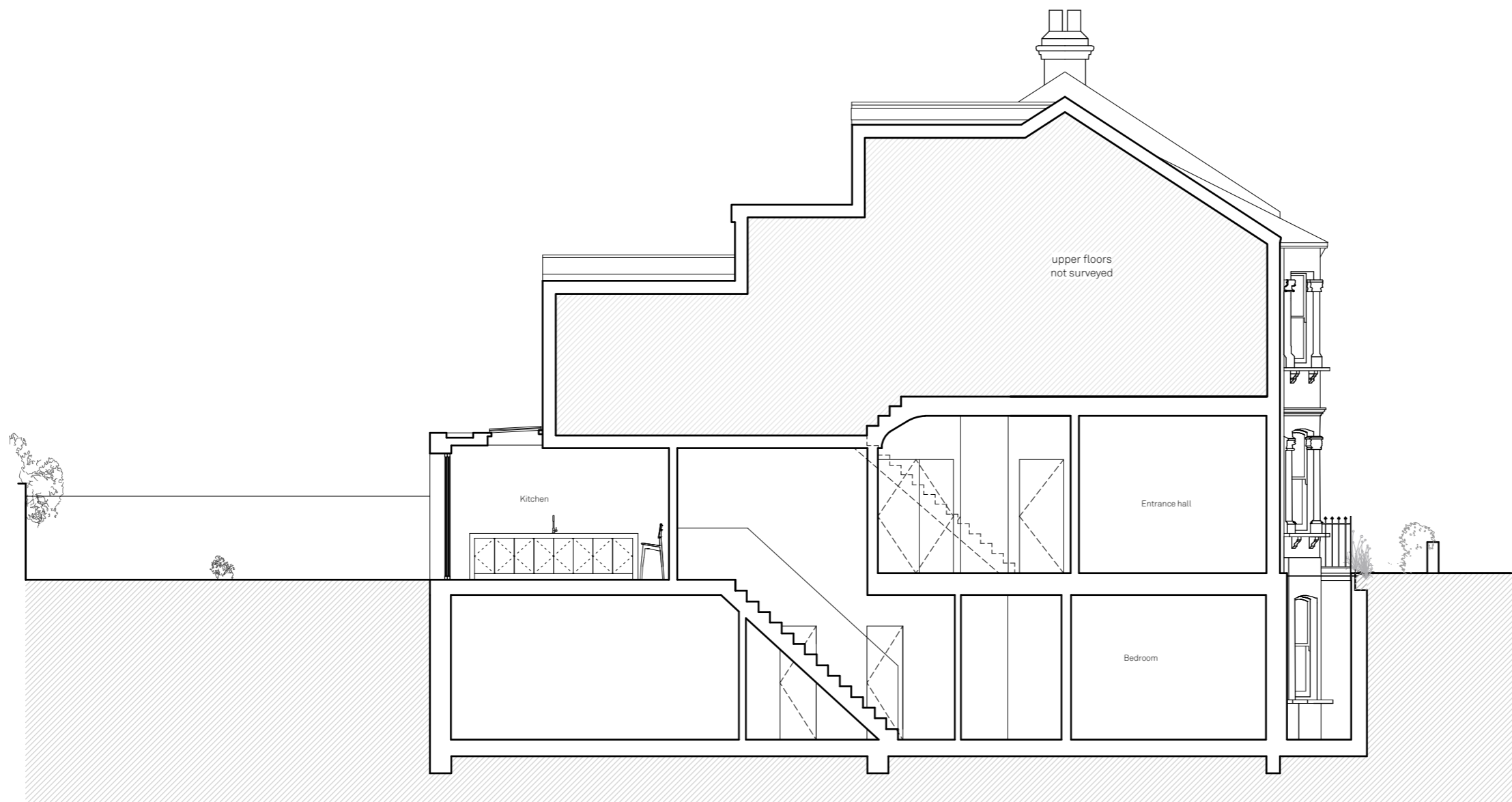
Section BB
