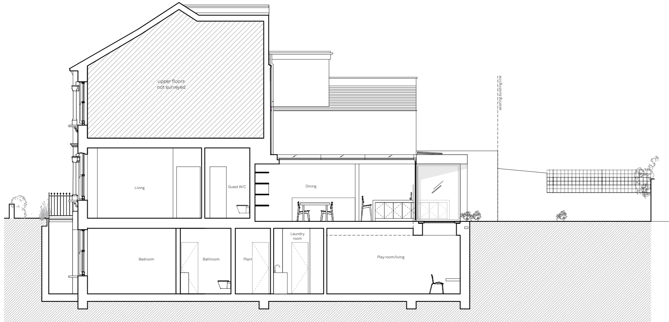
Section AA
