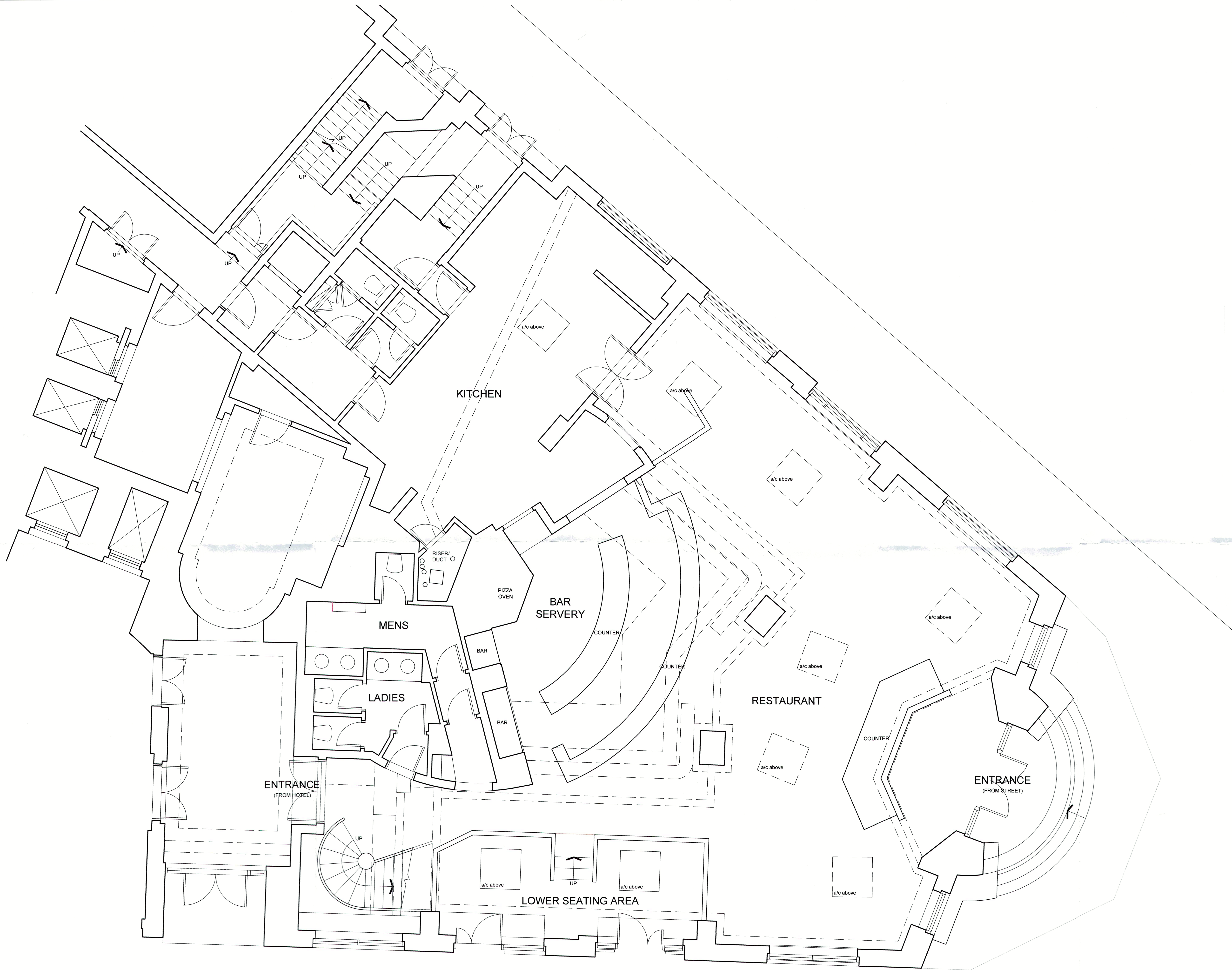
EXISTING GROUND FLOOR PLAN (RESTAURANT AREA) SCALE - 1:50
