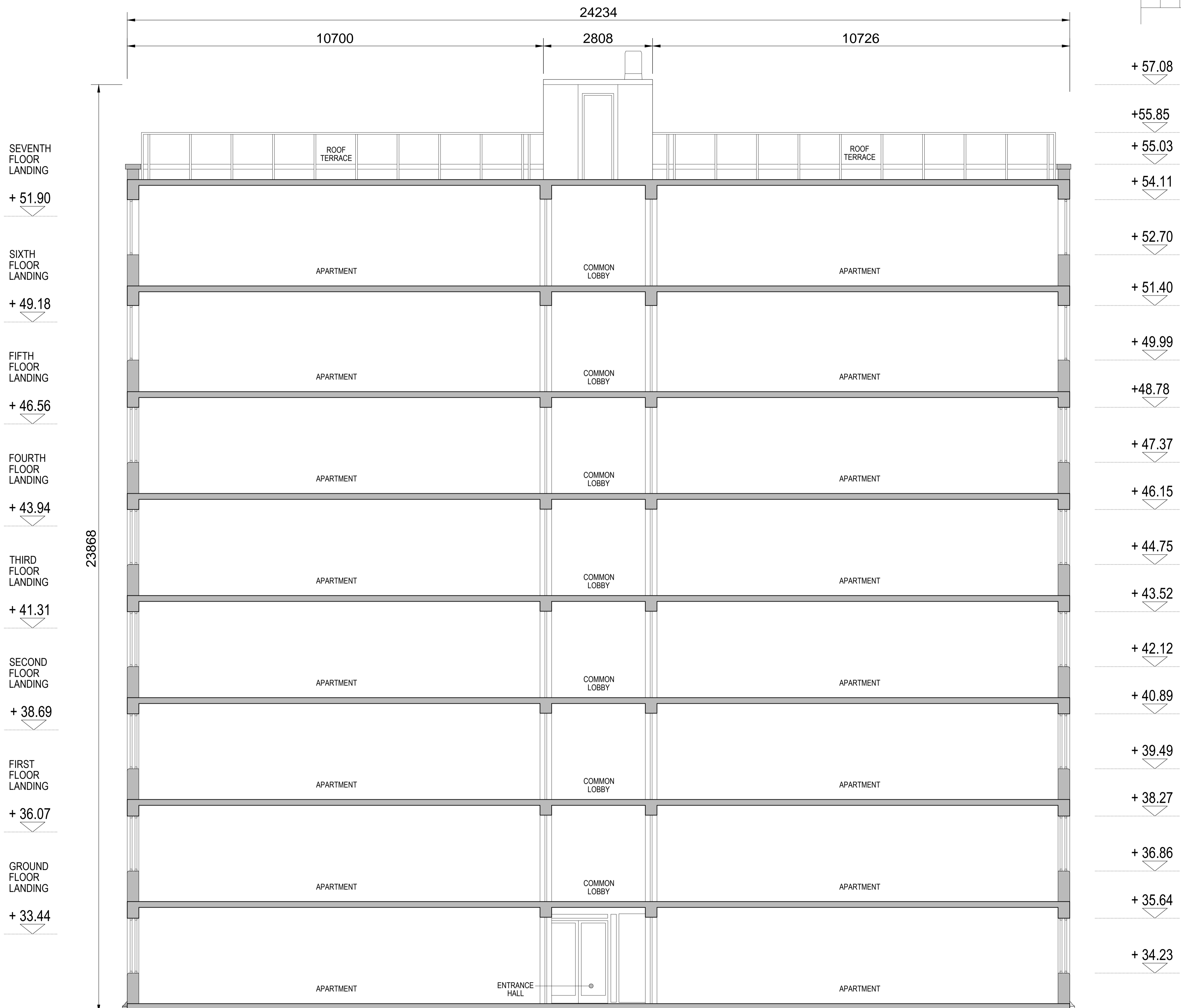
1 LONG SECTION 1:50
