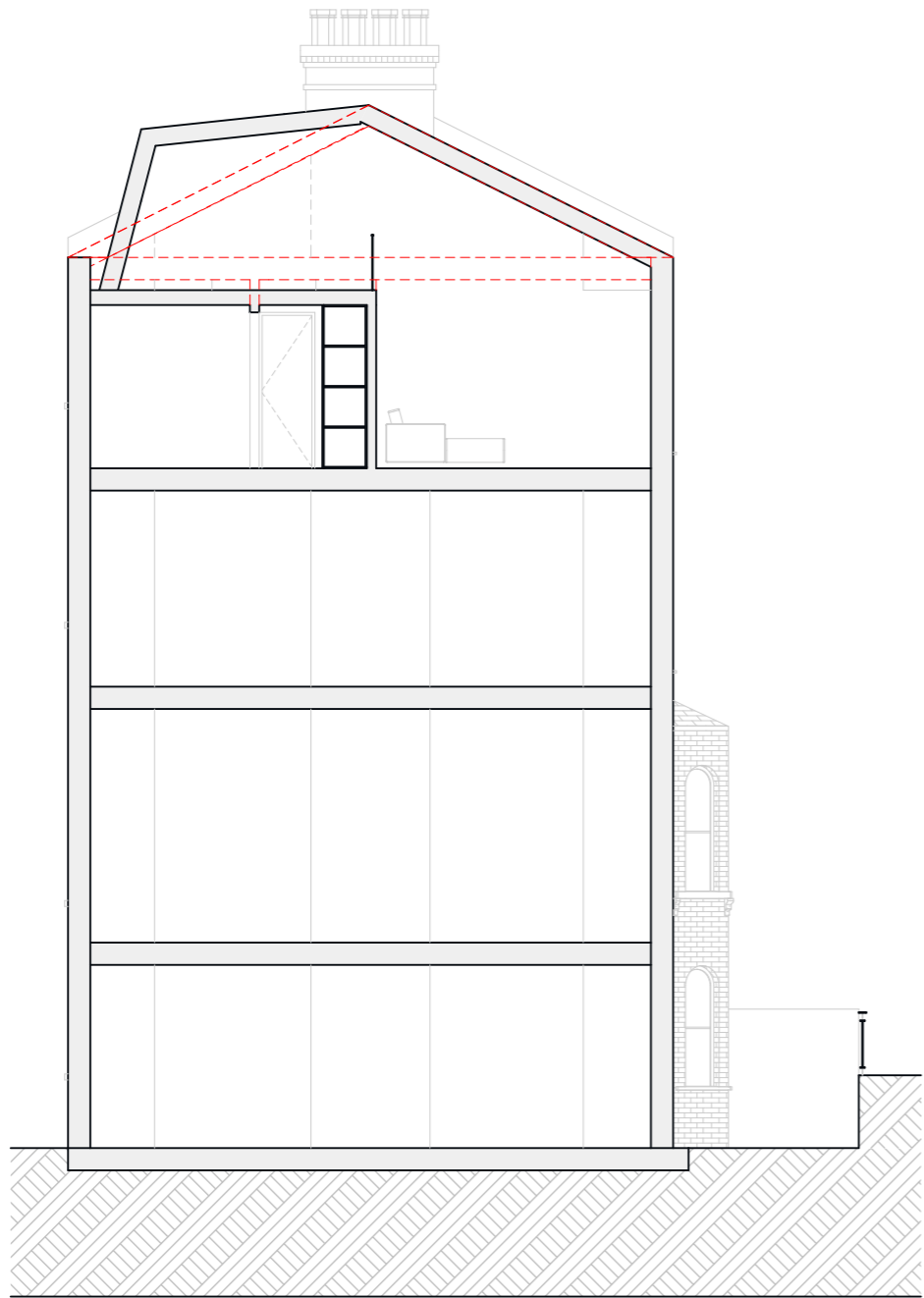
01 PROPOSED LONGITUDINAL SECTION 01 1:100
