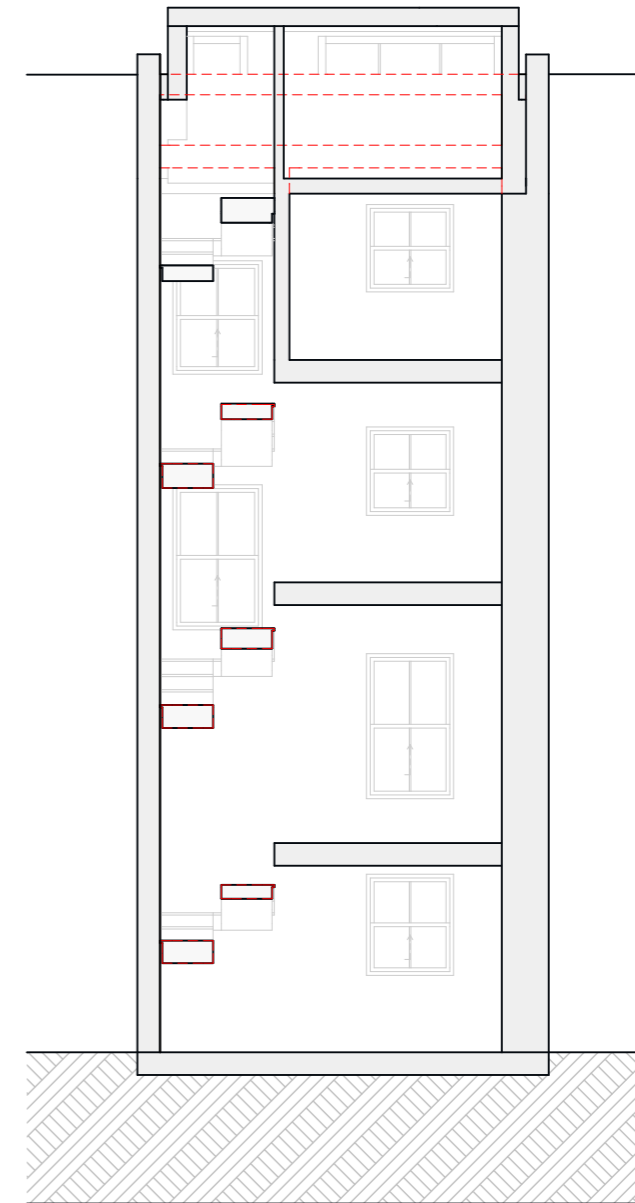
04 PROPOSED TRANSVERSAL SECTION 04 1:100
