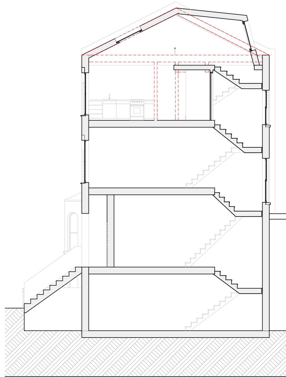
03 PROPOSED LONGITUDINAL SECTION 03 1:100
