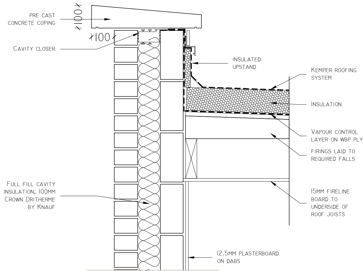
TYPICAL CAPPING DETAIL DT01/01
