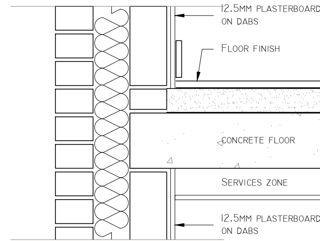
TYPICAL CONCRETE FLOOR DETAIL DT01/02
