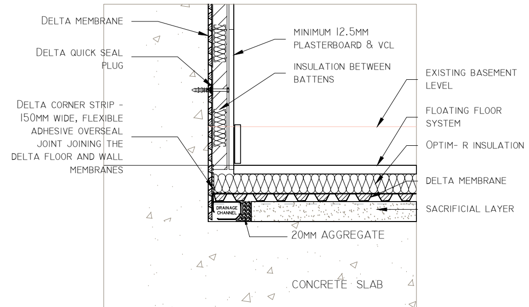
TYPICAL BASEMENT SLAB DETAIL DT01/05
