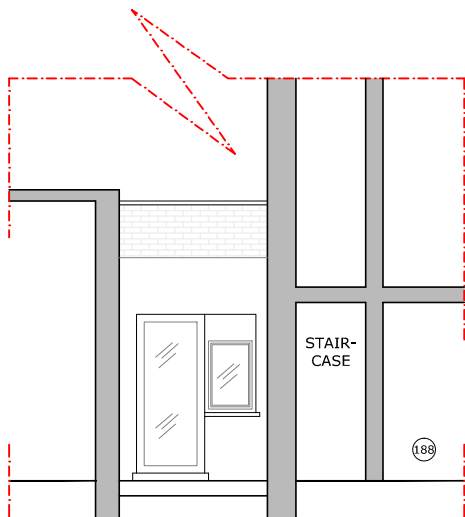
EXISTING SECTION B-B
