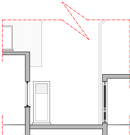
EXISTING SECTION A-A
