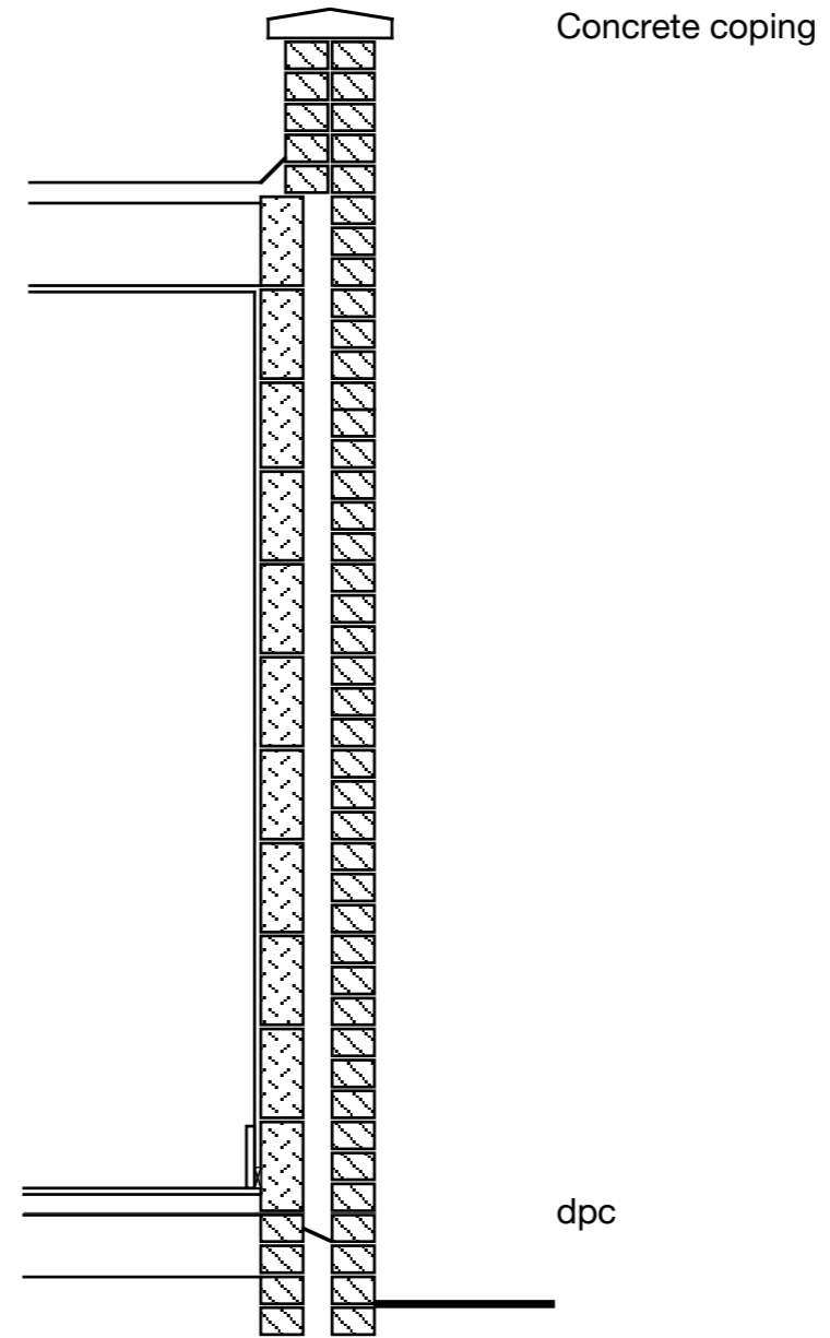
SECTION THROUGH WINDOW Scale 1:20
