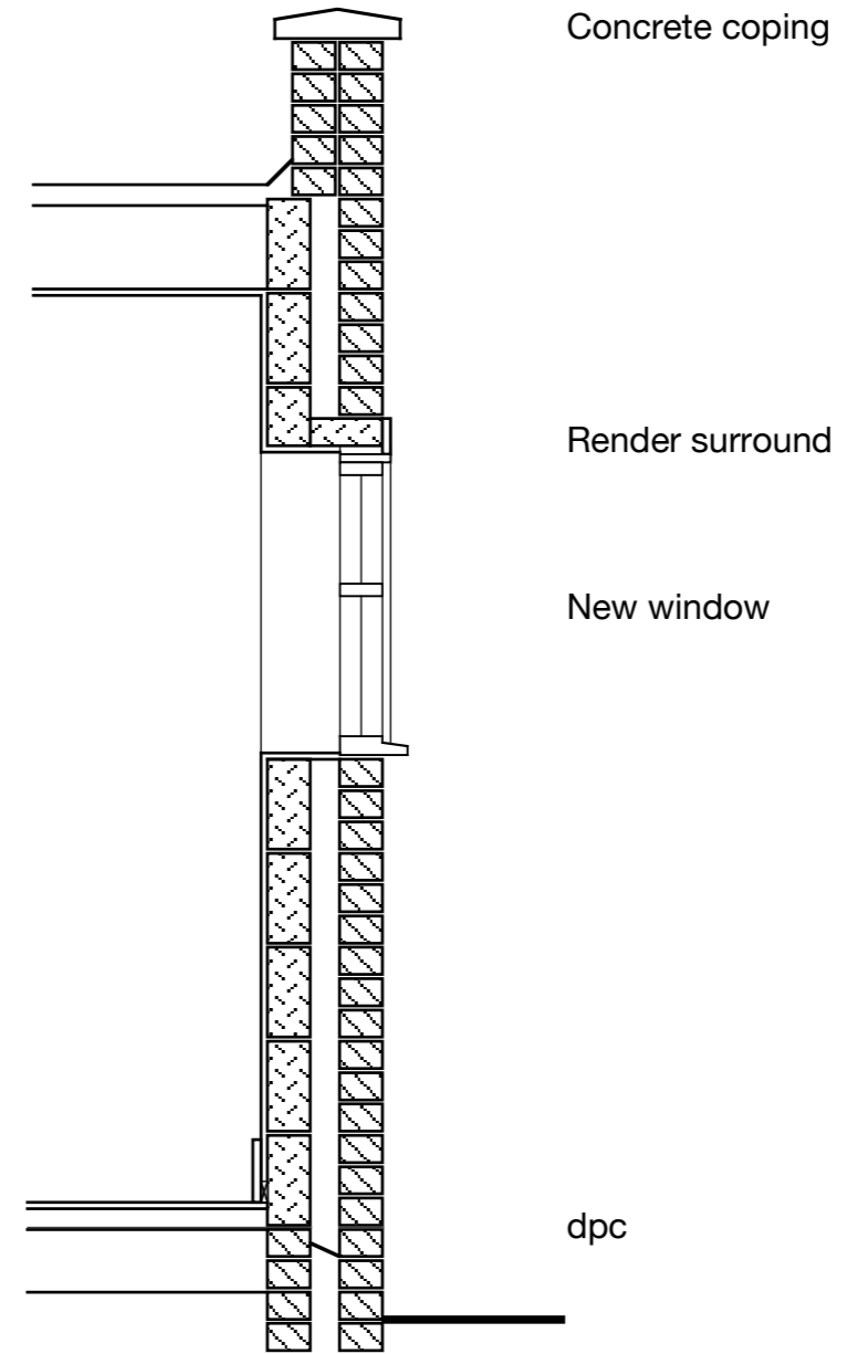
PROPOSED SECTION THROUGH WINDOW Scale 1:20
