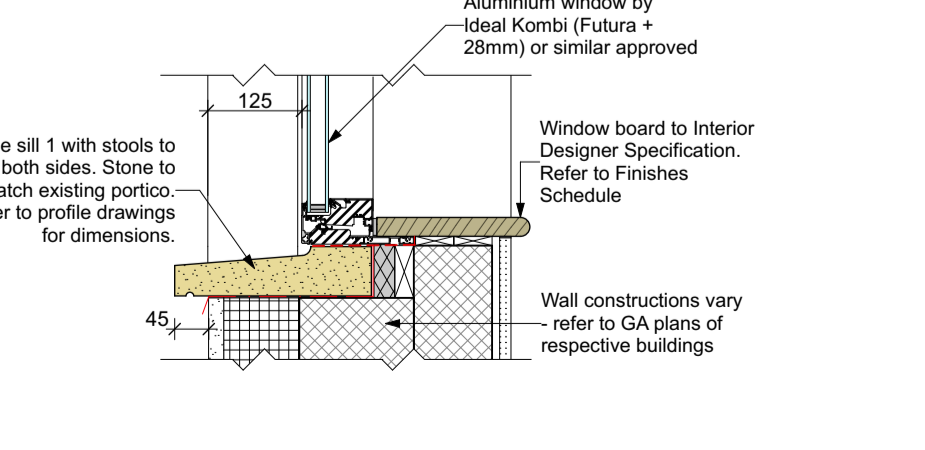
Detail SW6 - Stone sill detail to fixed aluminium window
