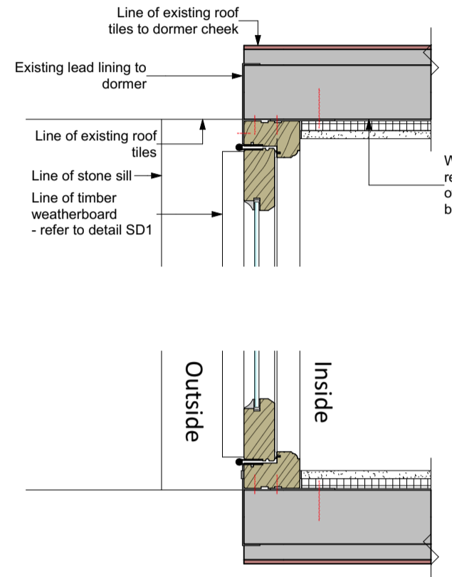
Detail J4 - Glazed door jamb to dormer window
