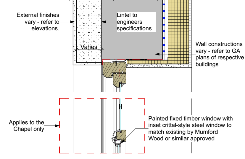
Detail H9 - Typical head detail to fixed window
