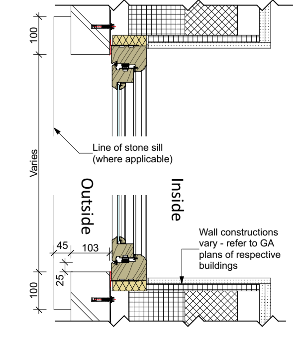
Detail J12 - Typical casement jamb in new brick wall
