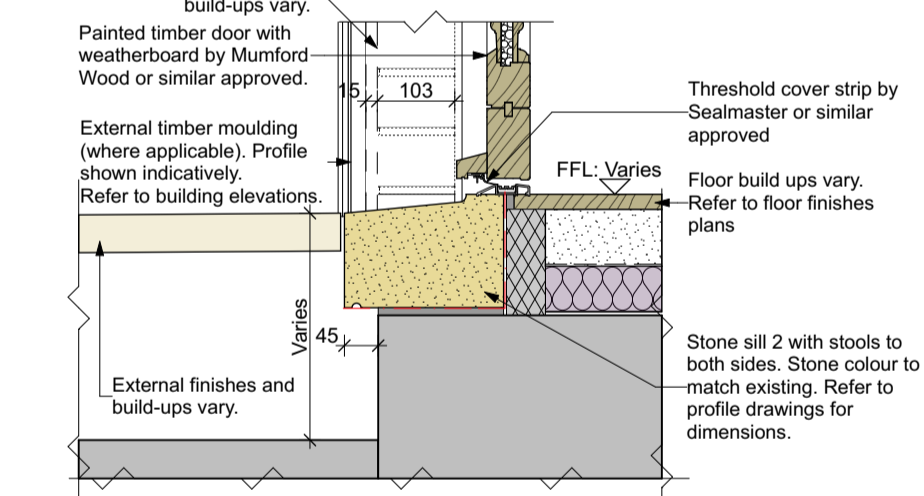
Detail SD2 - Typical panelled door to stone sill detail - ground floor entrance doors (opening in)
