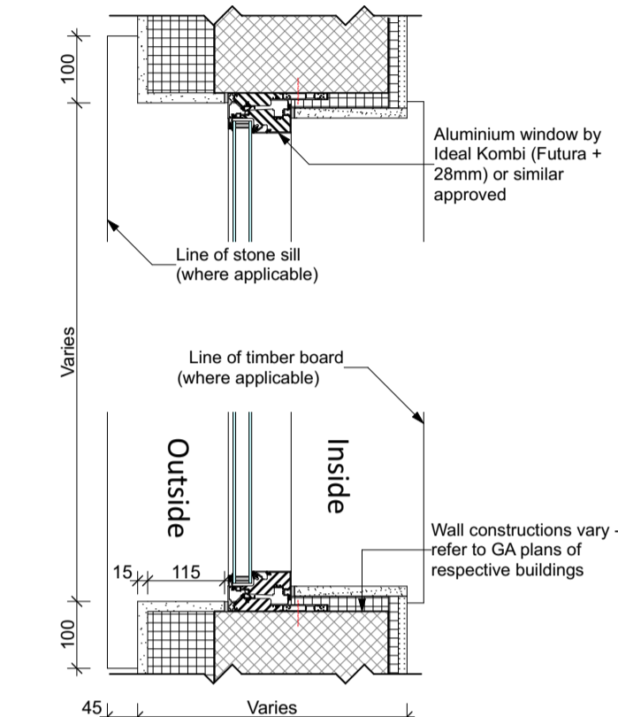
Detail J9 - Typical fixed window jamb in new wall
