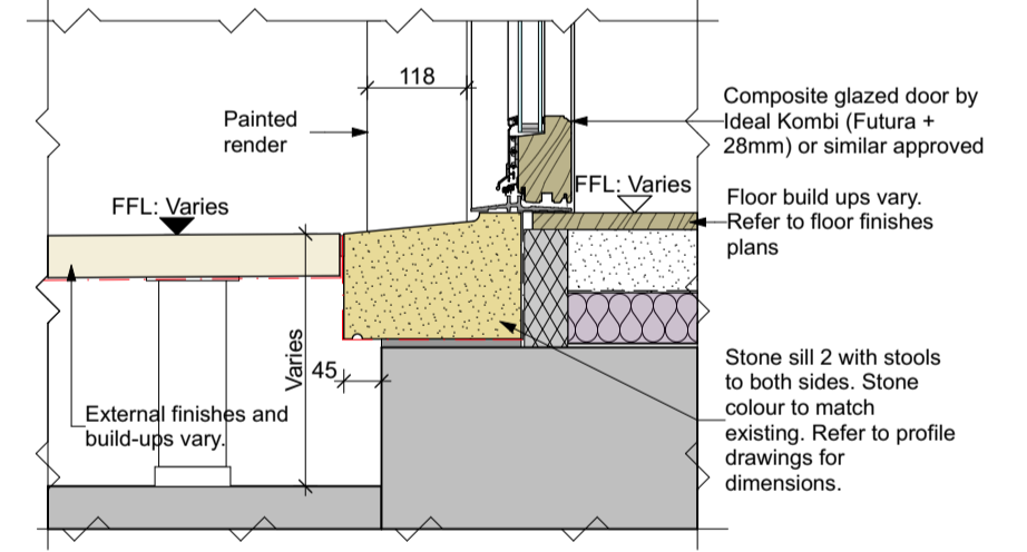
Detail SD5 - Typical glazed composite door to stone sill within rendered wall
