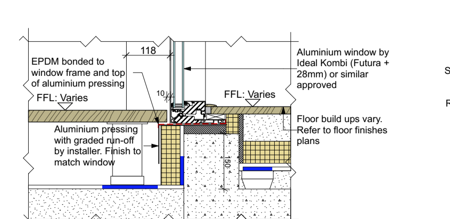
Detail SW5 - Typical fixed aluminium full height window sill
