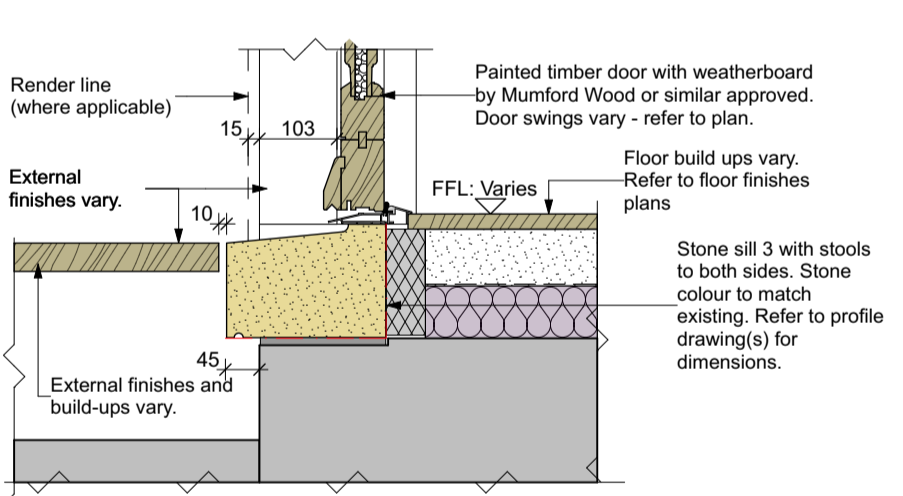
Detail SD2 - Typical panelled door to stone sill detail - ground floor entrance doors (opening out)
