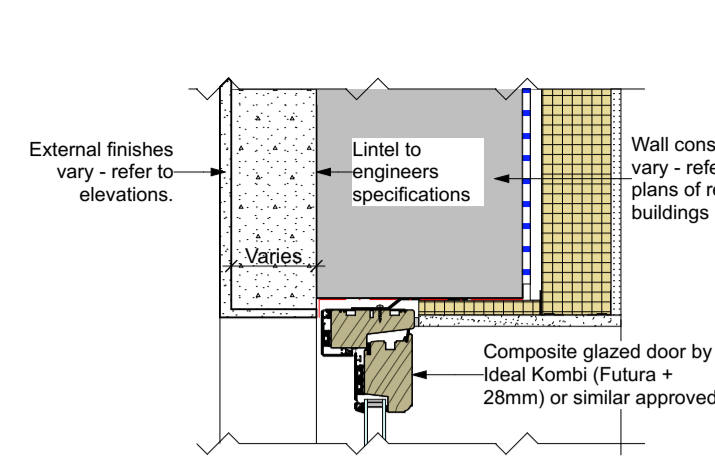
Detail H8 - Typical head detail to composite door
