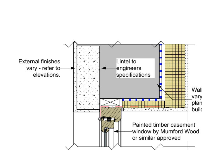
Detail H10 - Typical head detail to casement window
