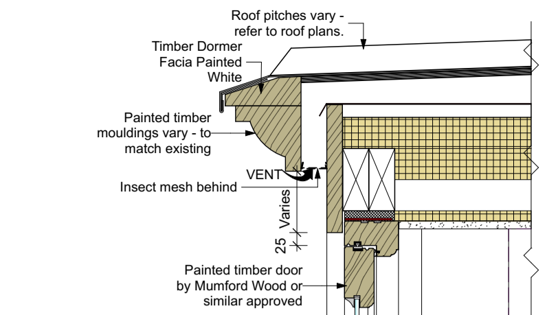
Detail H6 - Typical head detail to door within dormer
