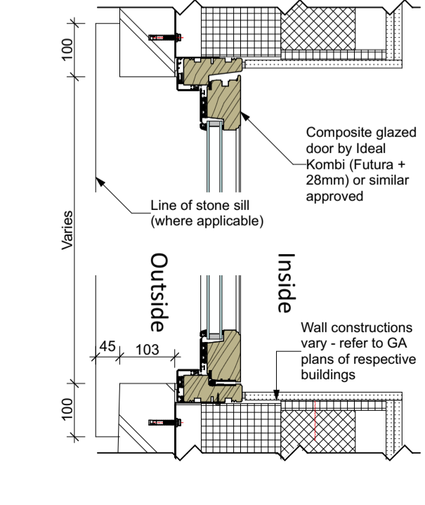
Detail J11 - Typical glazed door jamb in new brick wall
