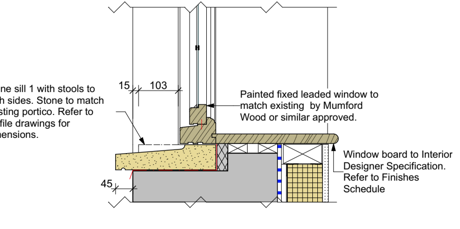
Detail SW4 - Stone sill detail to fixed window
