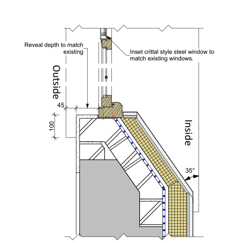
Detail J5 - Chapel fixed window jamb with splayed reveal
