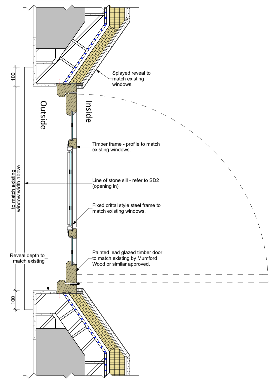
Detail J8 - Chapel splayed reveal door jamb
