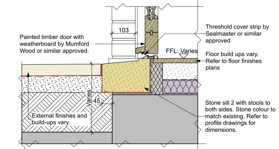
Detail SD3 - Typical panelled door within brick wall to stone sill detail
