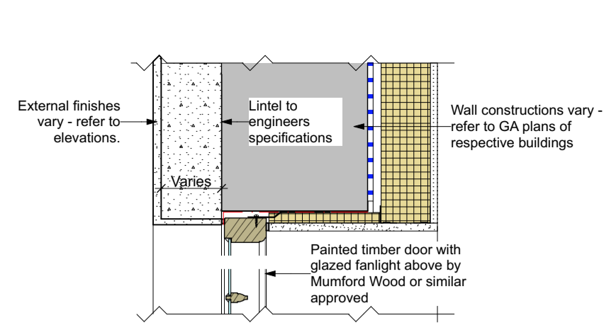
Detail H5 - Typical head detail to fixed fanlight
