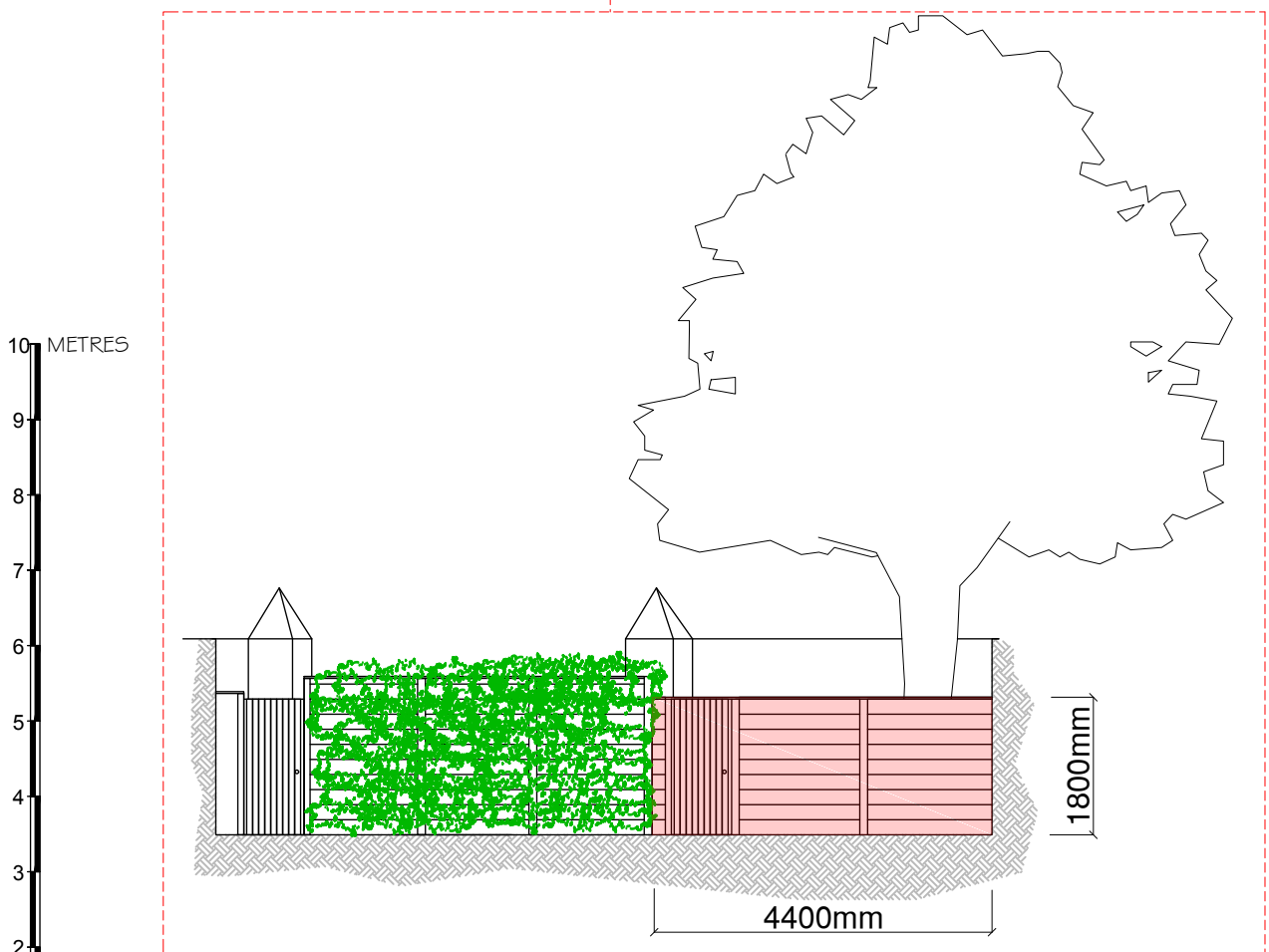
Proposed timber panel fence in front garden Elevation
