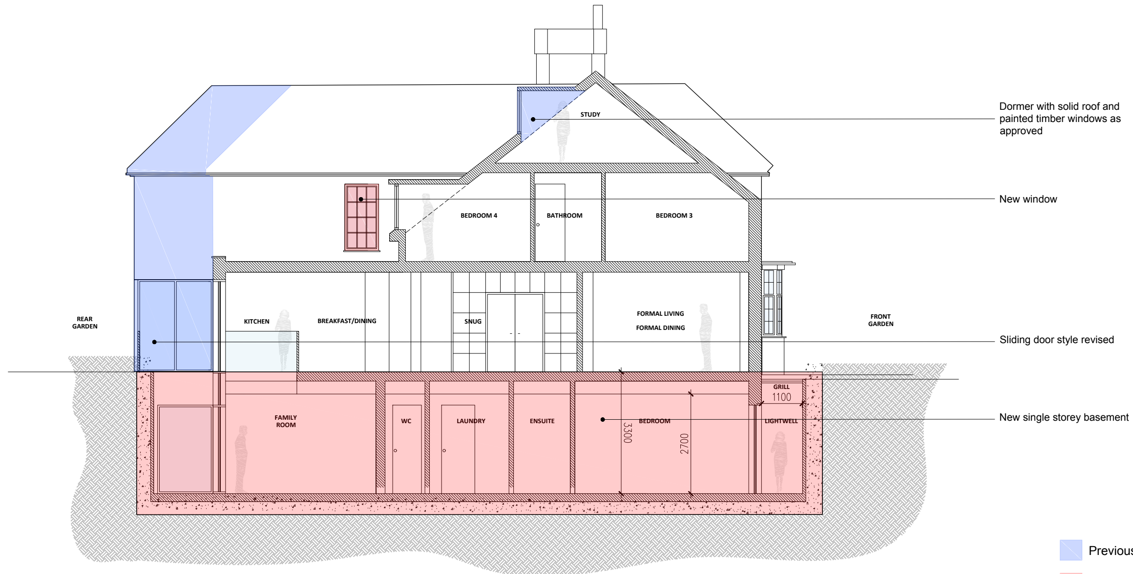
PROPOSED LONG SECTION - D
