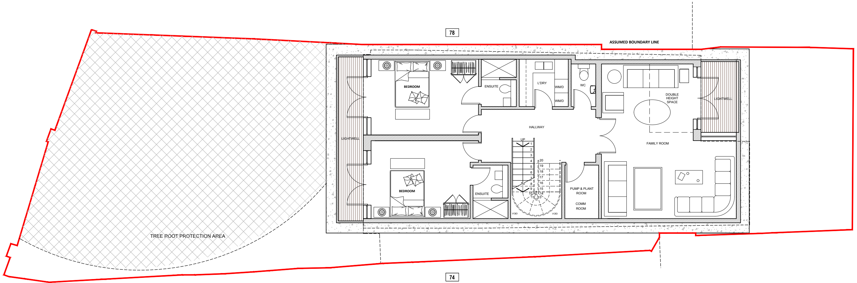
PROPOSED BASEMENT FLOOR PLAN
