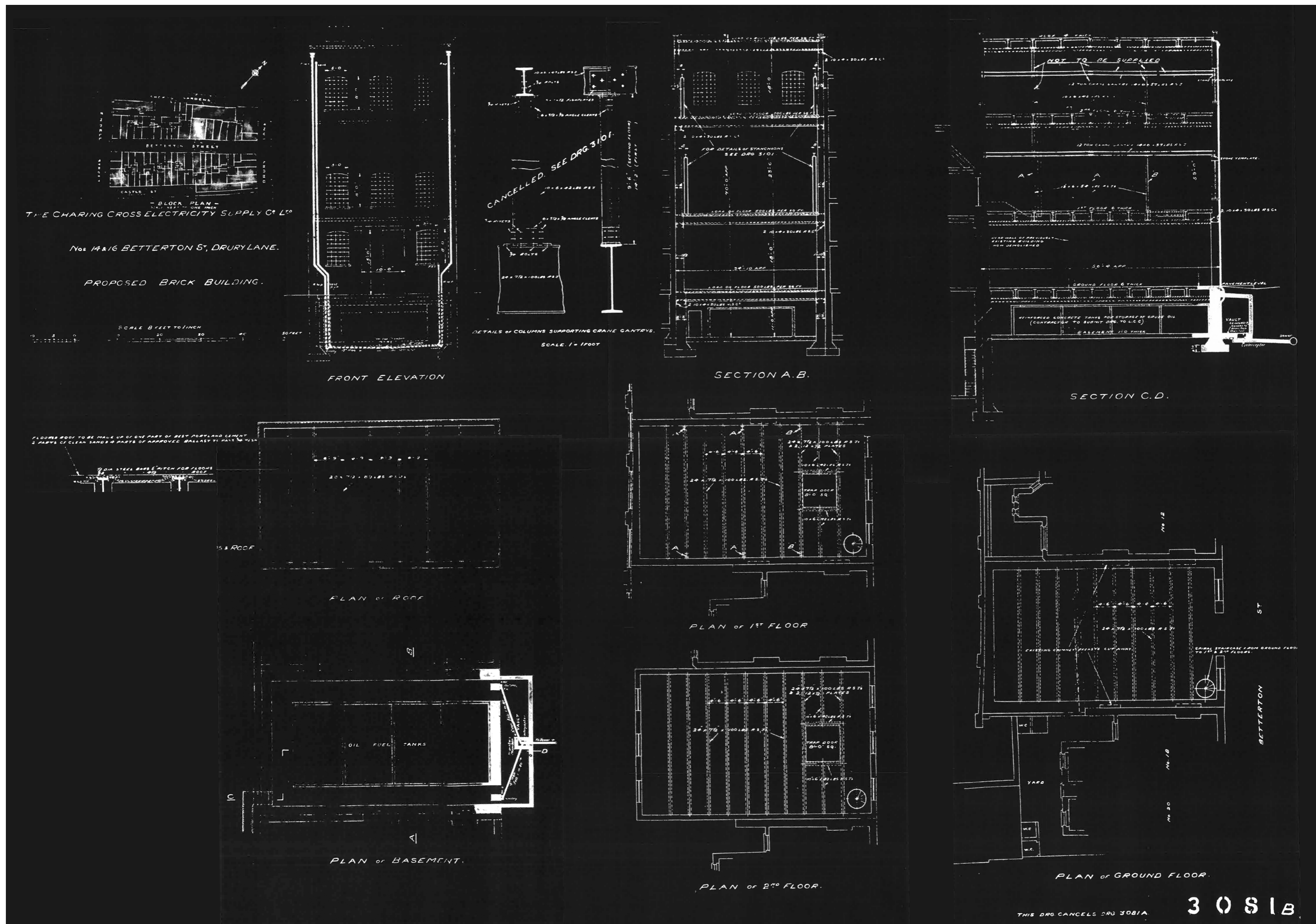
Figure A5.3: Drainage Application for 14-16 Betterton Street (1927)
