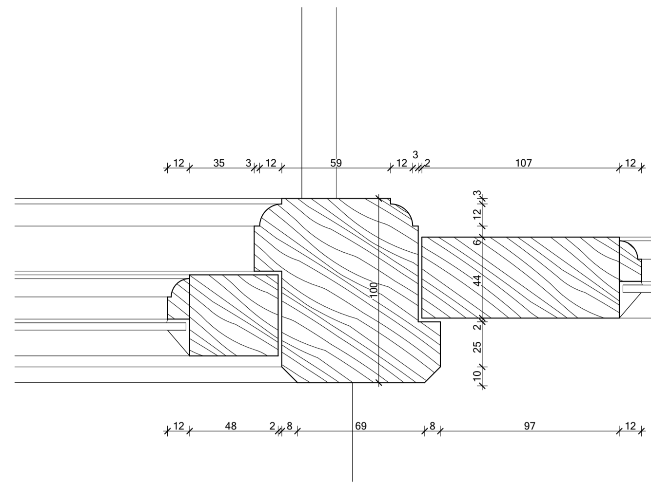
02 Mullion detail as extg
