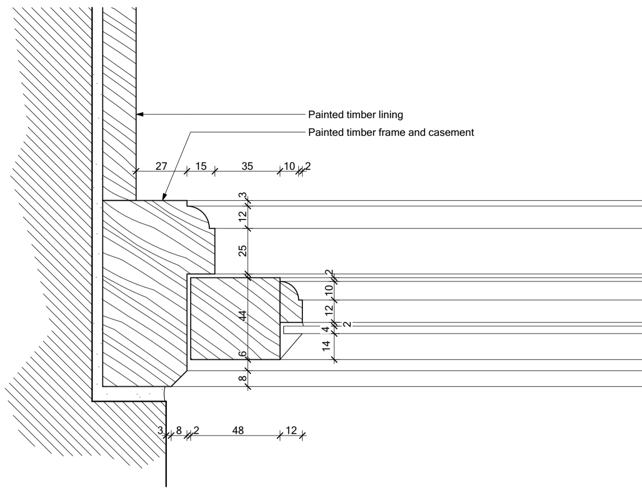
01 Jamb detail as extg
