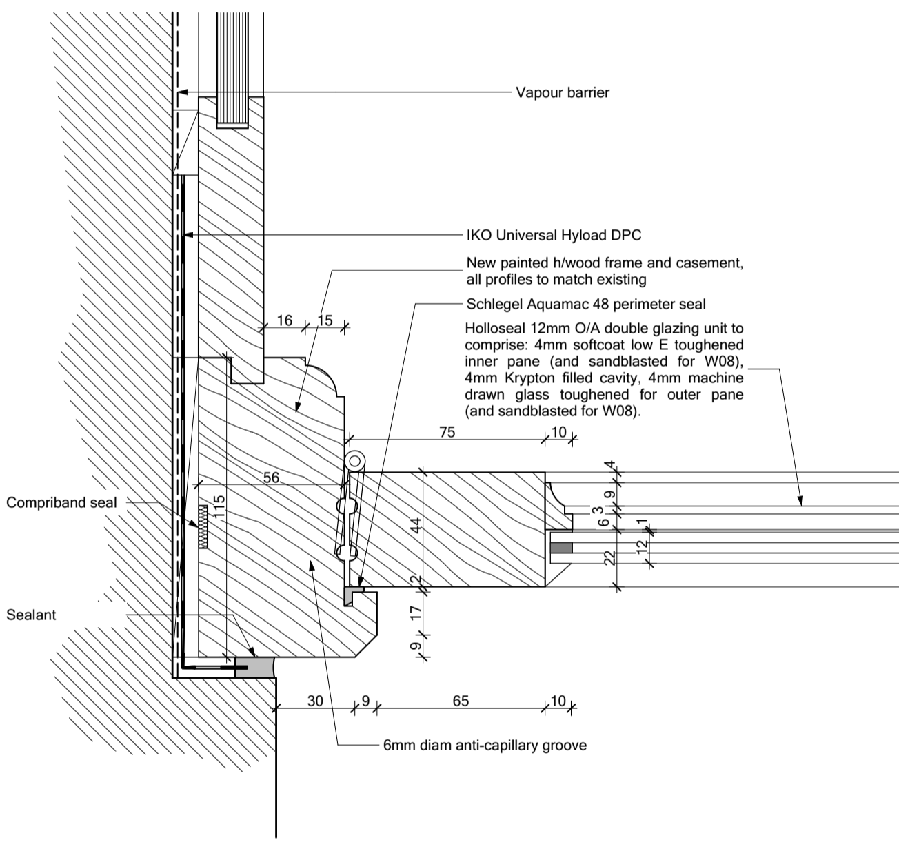
03 Jamb detail as proposed
