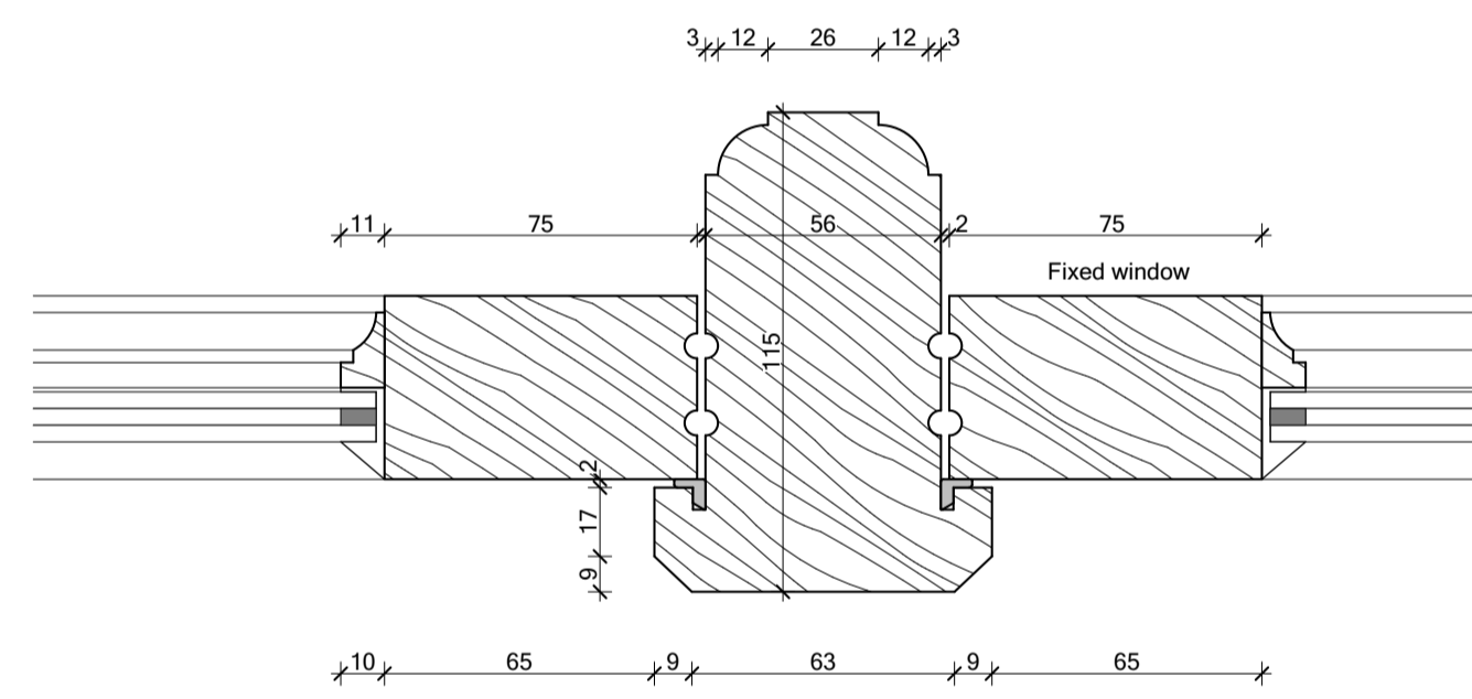
04 Mullion detail as proposed
