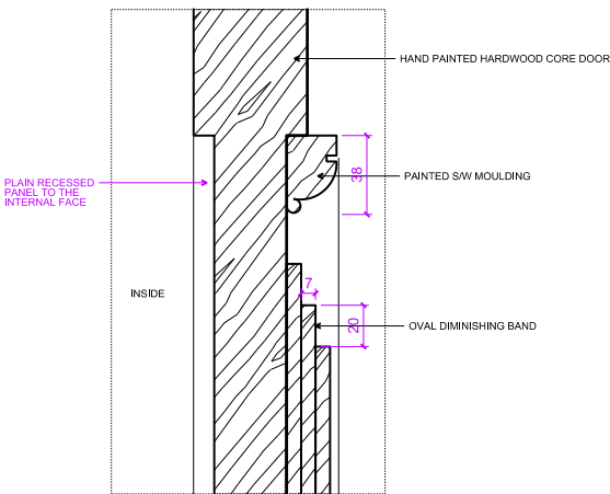
02 MOULDING DETAIL
