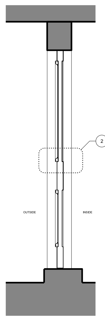
06 LOWER FRONT DOOR SECTION
