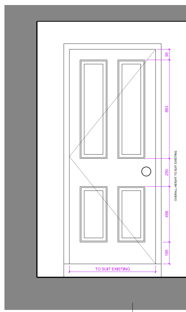
05 PROPOSED LOWER FRONT DOOR
