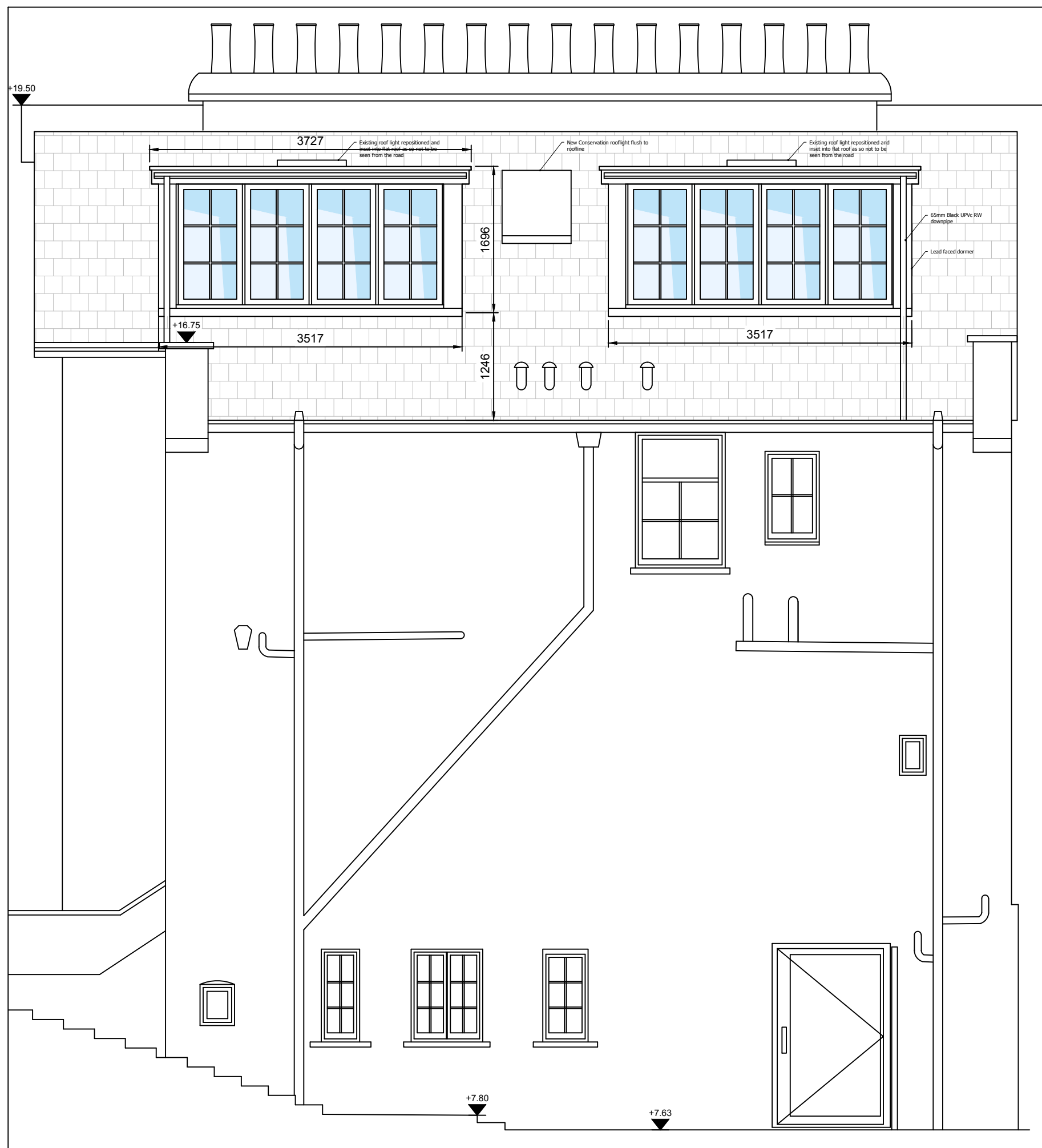
SIDE ELEVATION AS PROPOSED 1:50 @ A3
