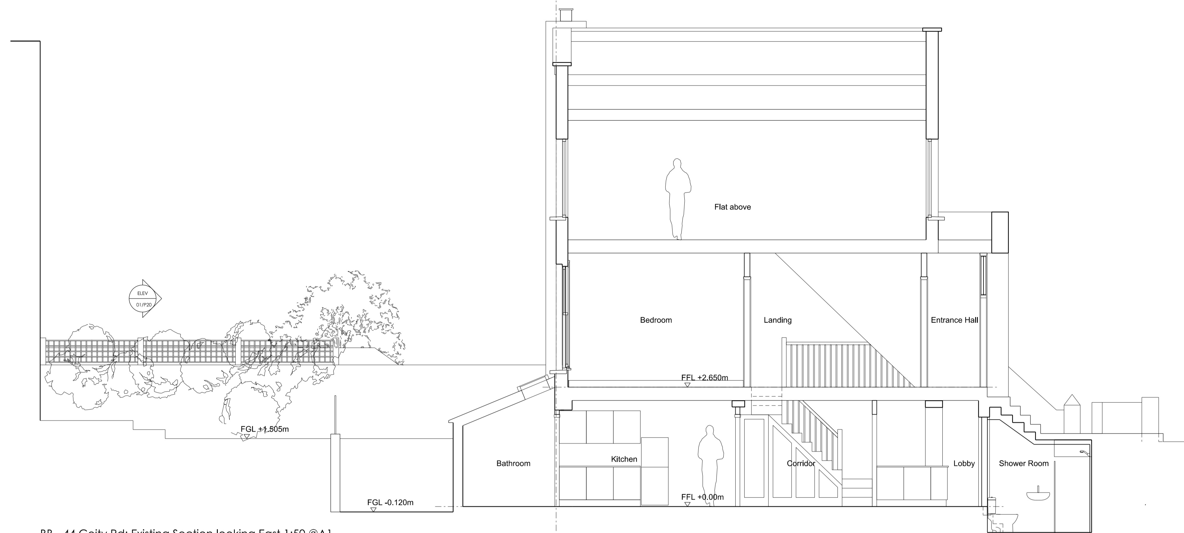
BB - 44 Coity Rd: Existing Section looking East 1:50 @A1
