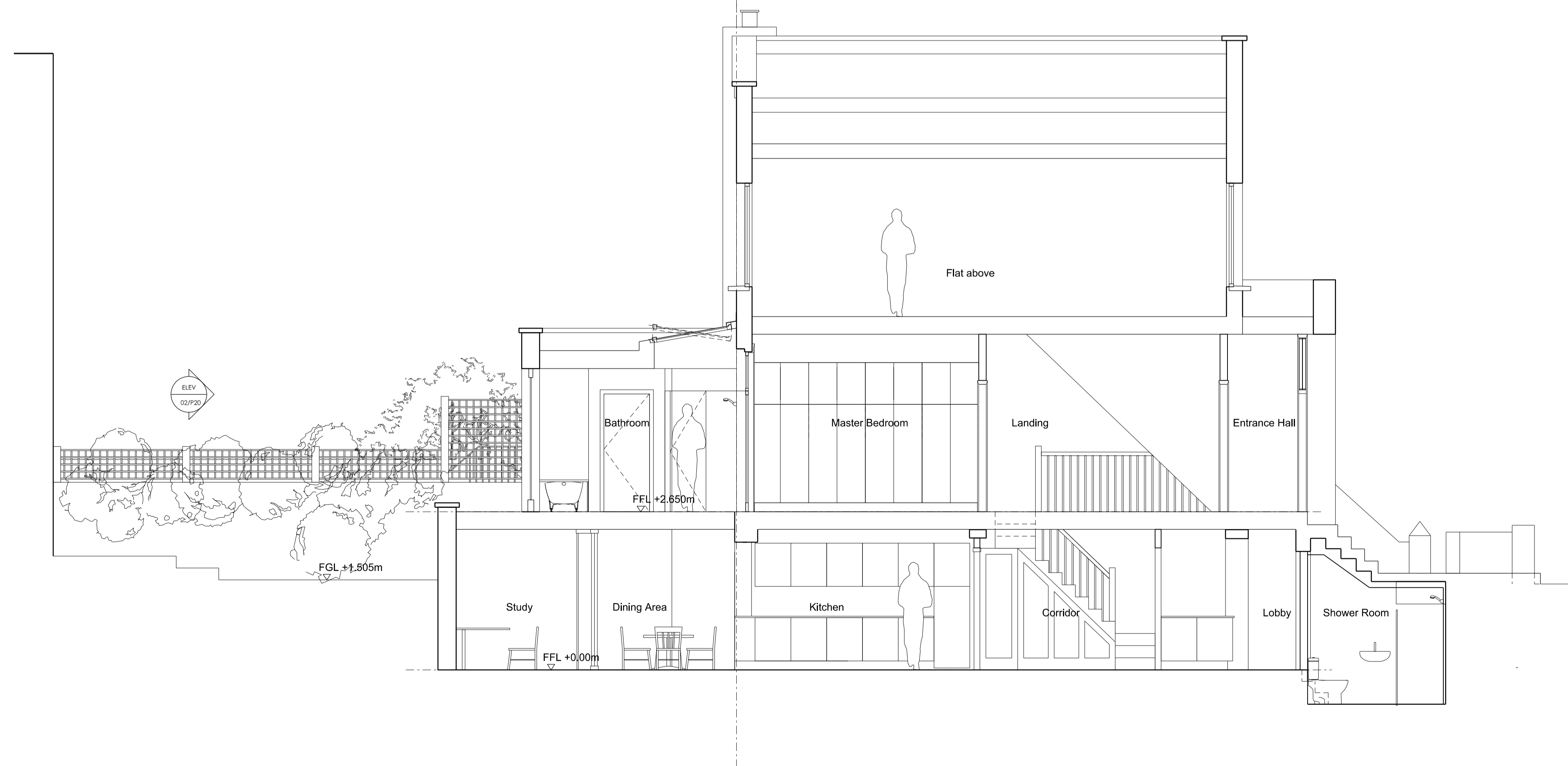
BB - 44 Coity Rd: Proposed Section Looking East 1:50 @A1
