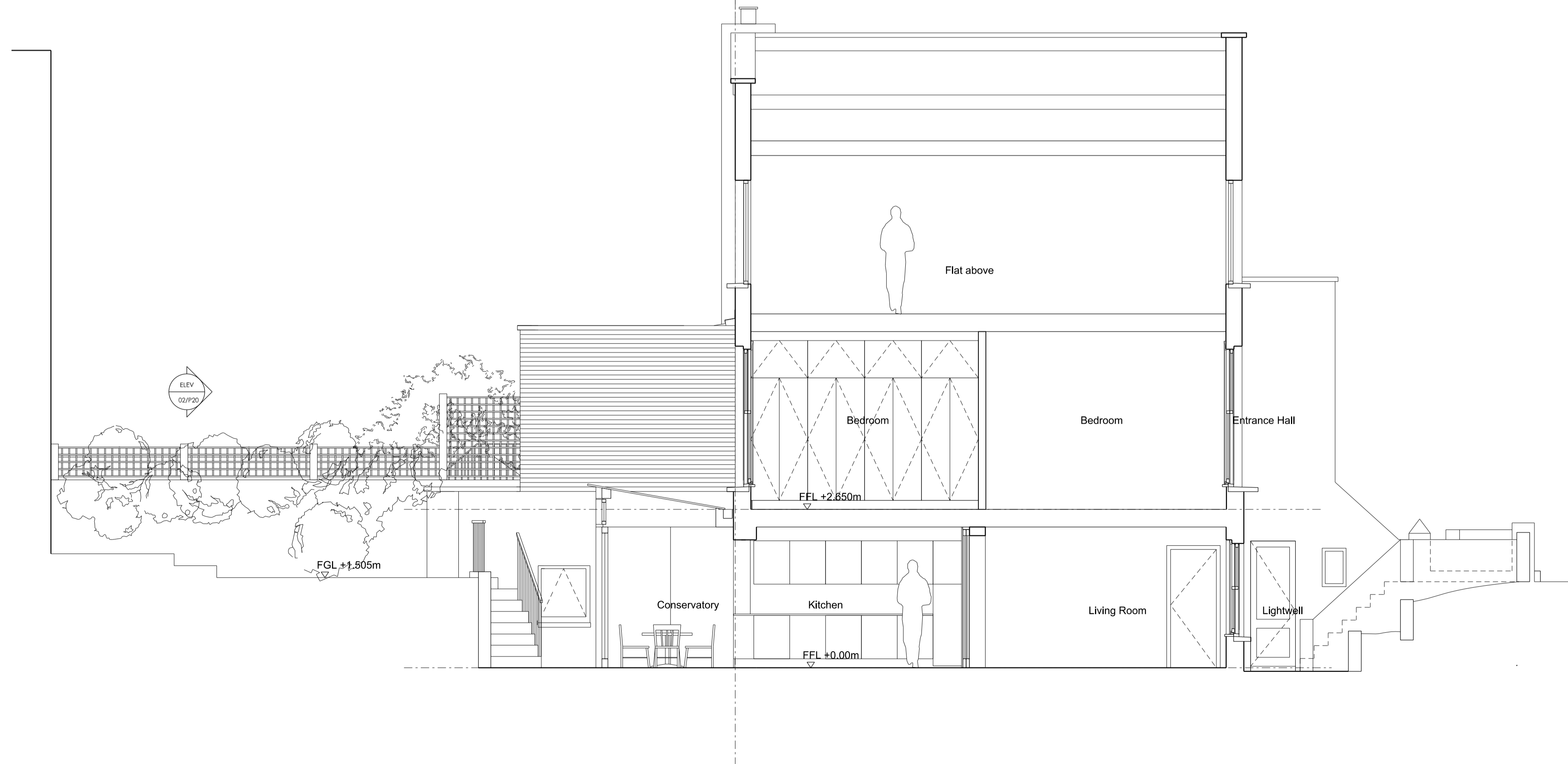
CC - 44 Coity Rd: Proposed Section Looking East 1:50 @A1
