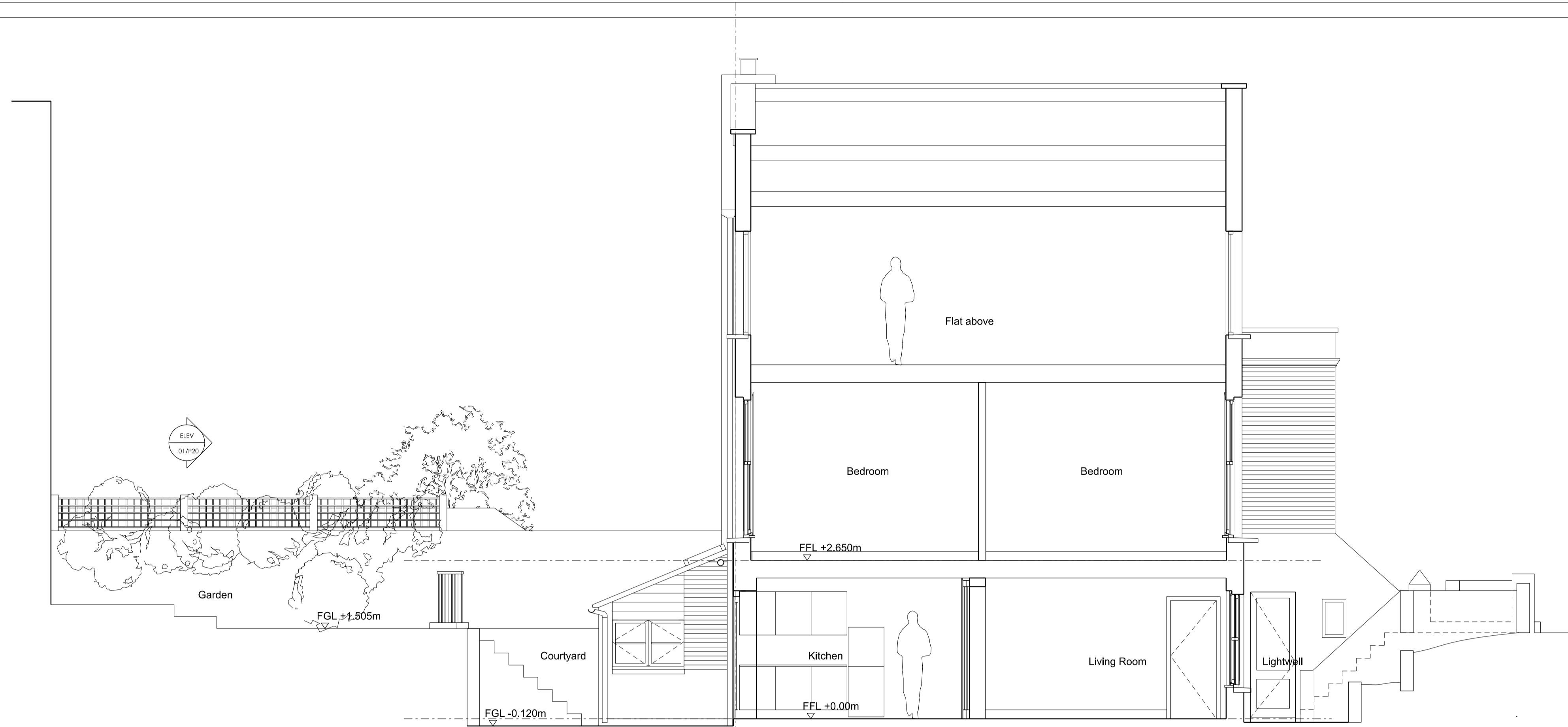
CC - 44 Coity Rd: Existing Section looking East 1:50 @A1
