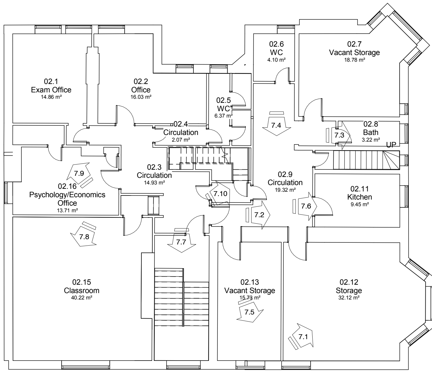
Second Floor Photo Plan 1 : 100
