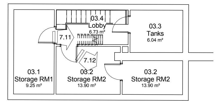
Third Floor Photo Plan 1 : 100
