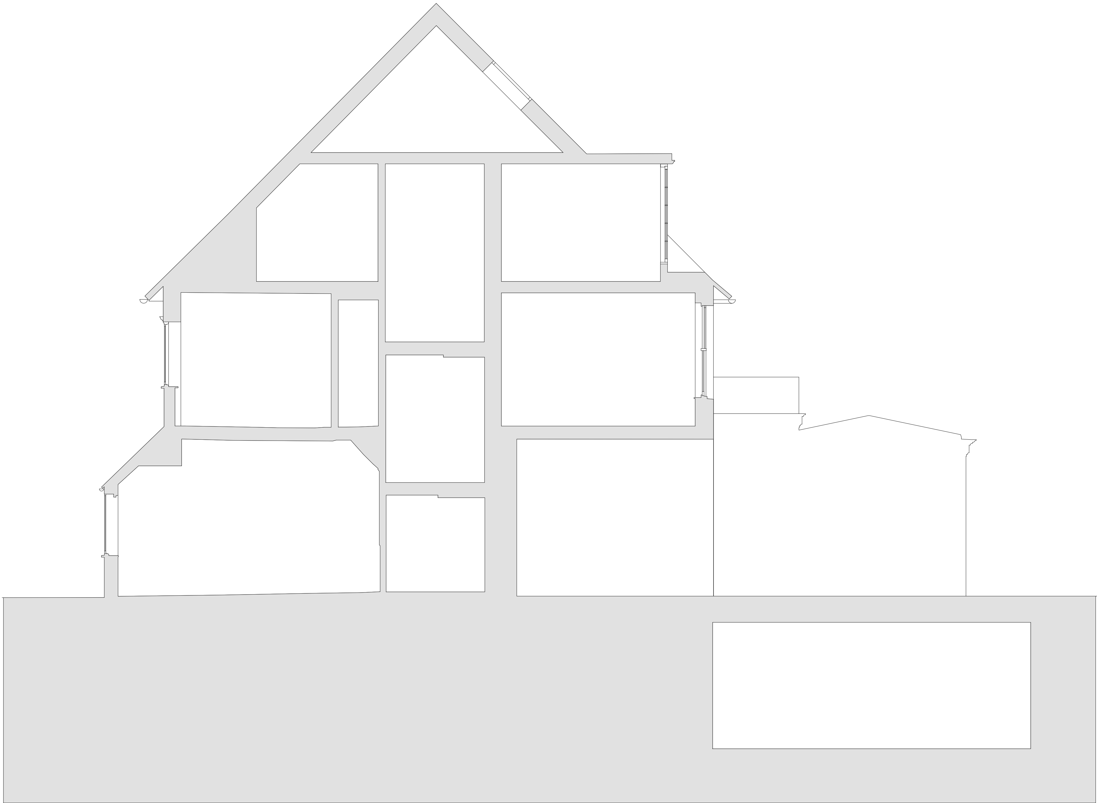
Sectional Elevation 1:50
