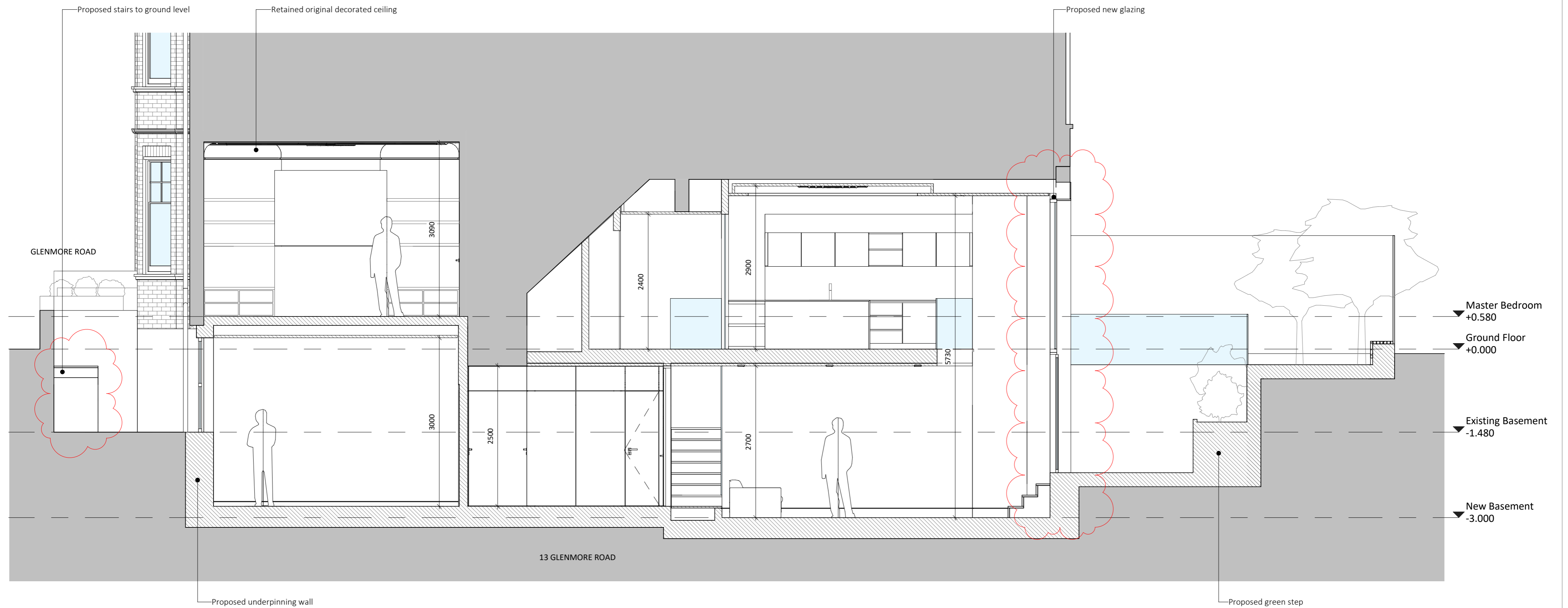
B Proposed Section B-B 1 : 50
