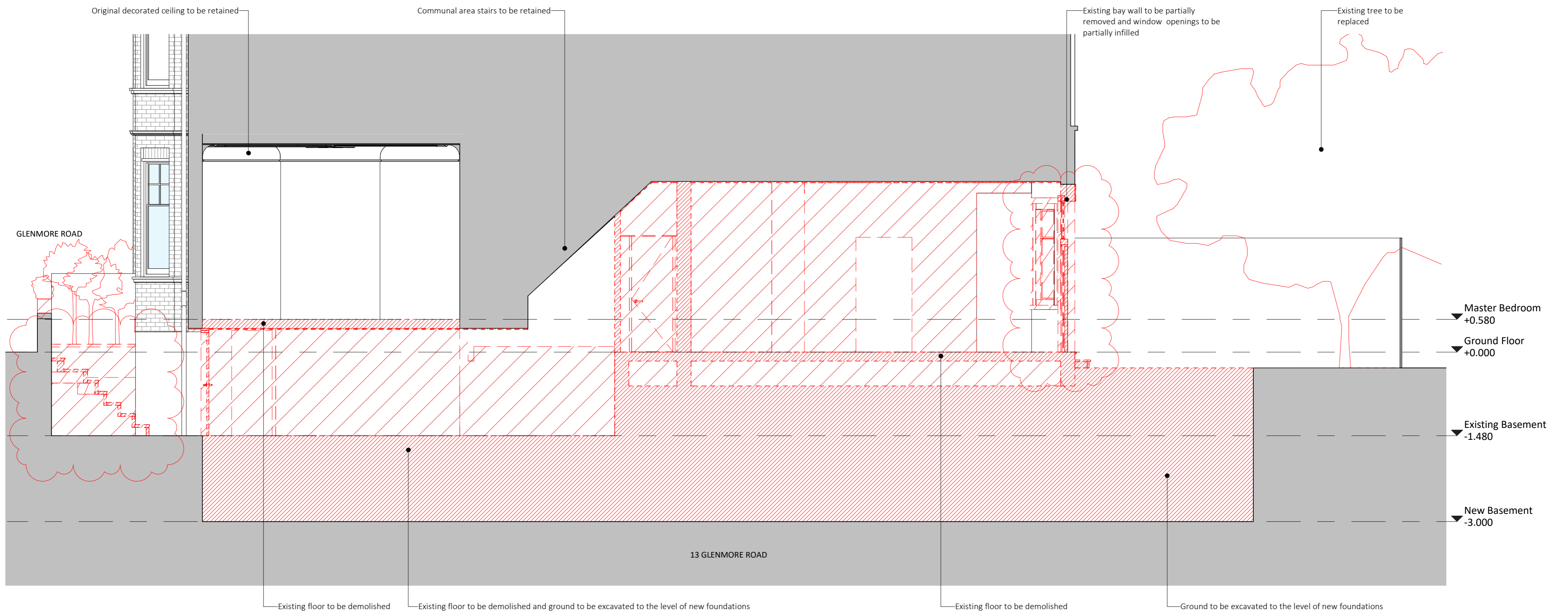
B Demolition Section B-B 1:50
