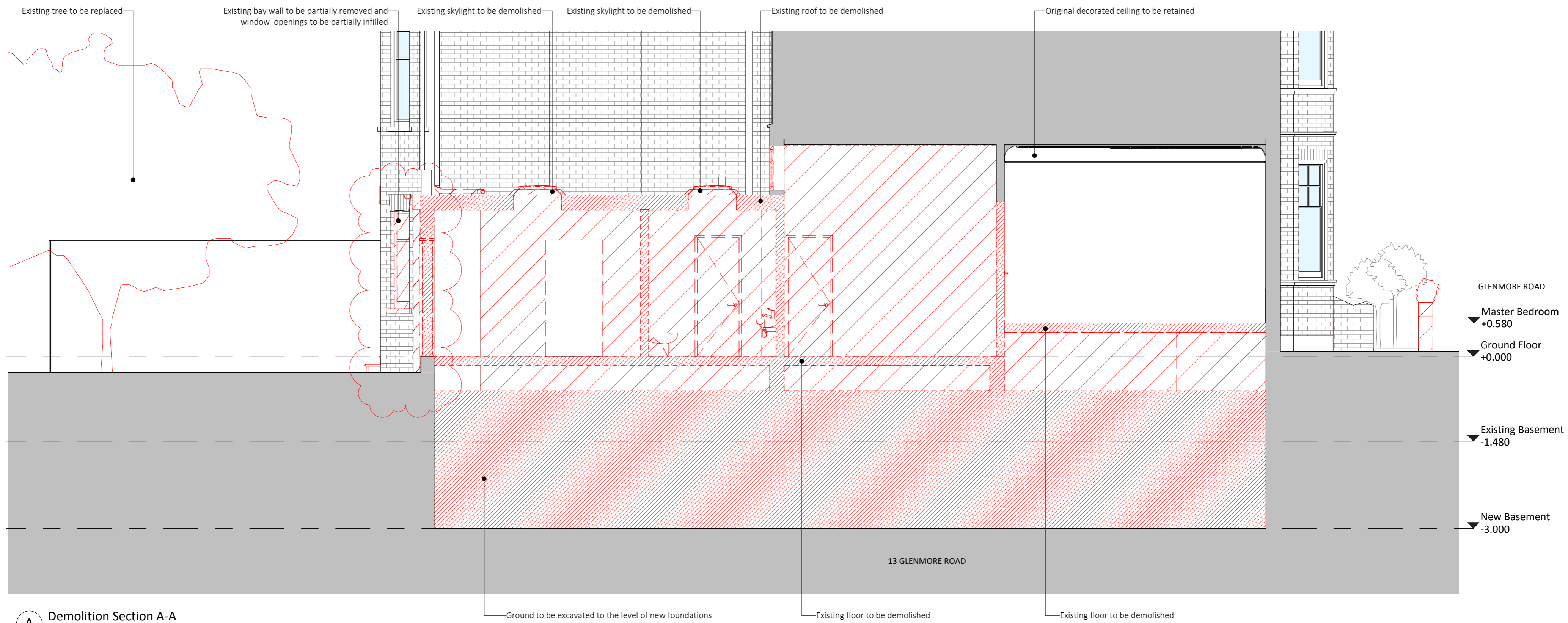
A Demolition Section A-A 1:50
