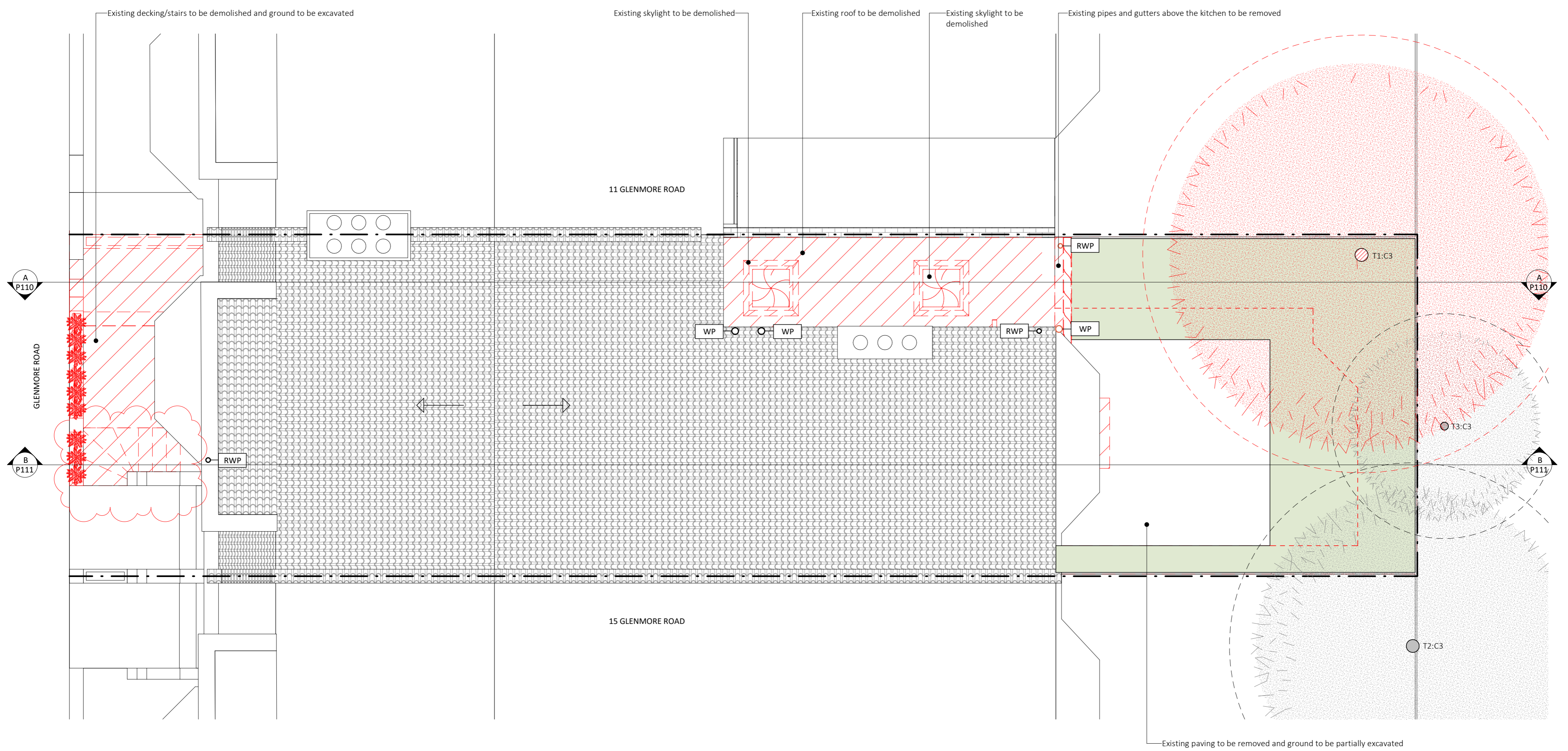
1 Demolition Roof Plan 1 : 50
