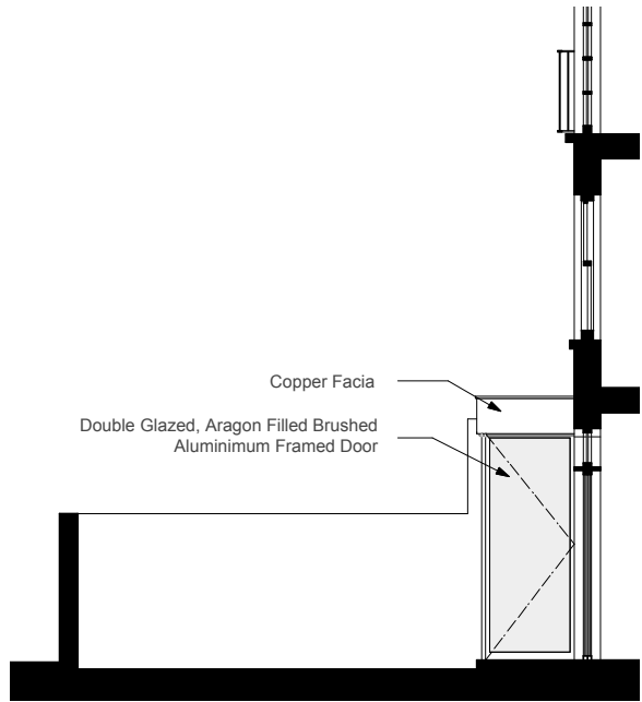
3 PROPOSED ELEVATION - 3
