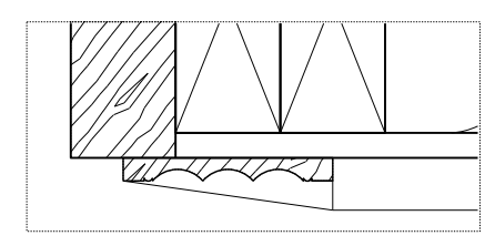
04 1:2 TYPICAL REEGED ARCHITRAVE
