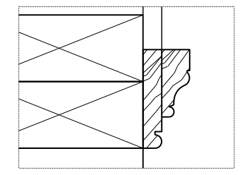
06 1:2 TYPICAL STANDARD ARCHITRAVE
