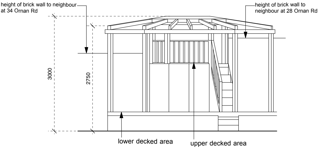
Xtg Plan & Elevation Of Single Storey Wooden Outbuilding & Decking 1:50 @ A3
