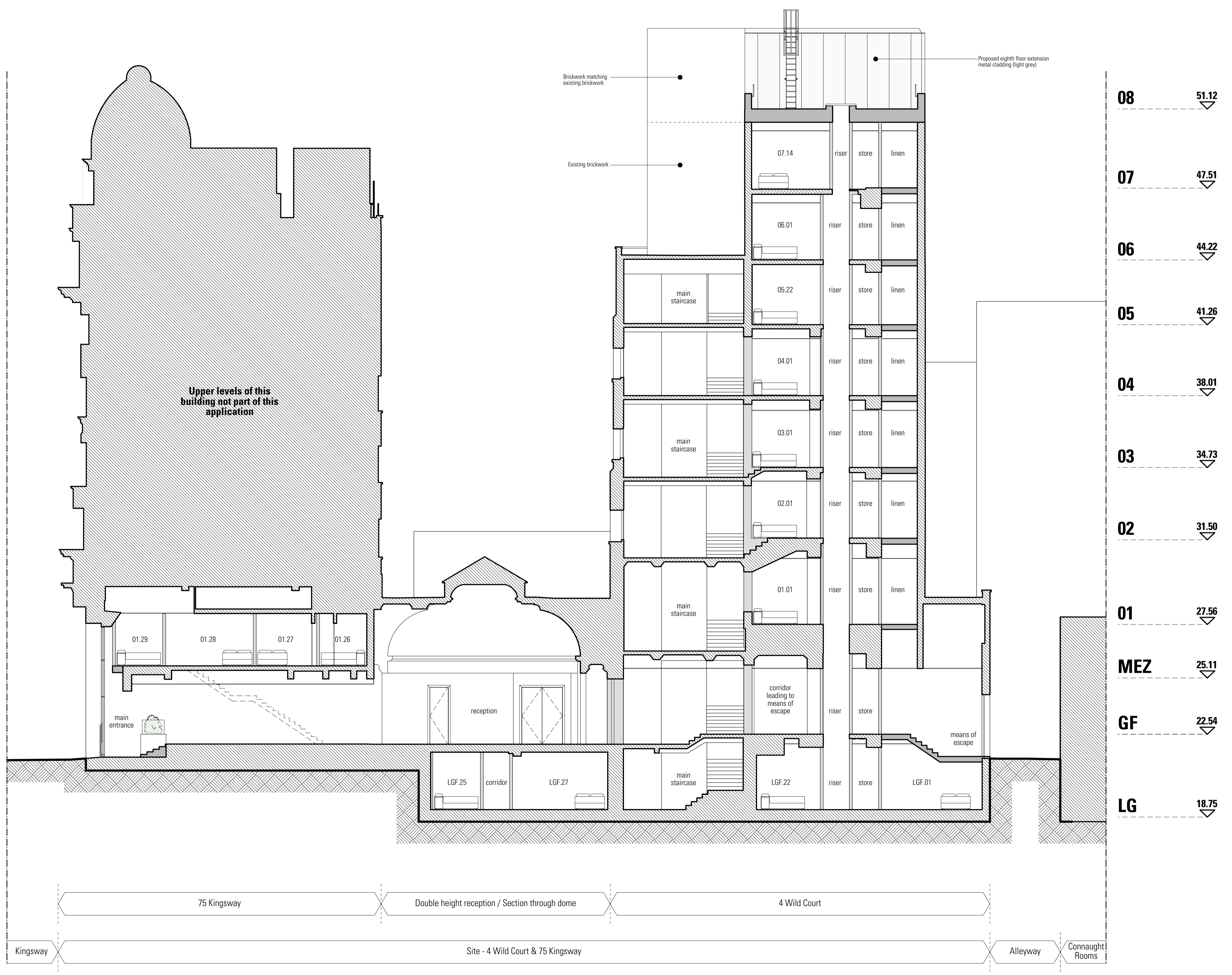
03 Proposed Section AA' Scale 1:100 @ A1 / 1:200 @ A3
