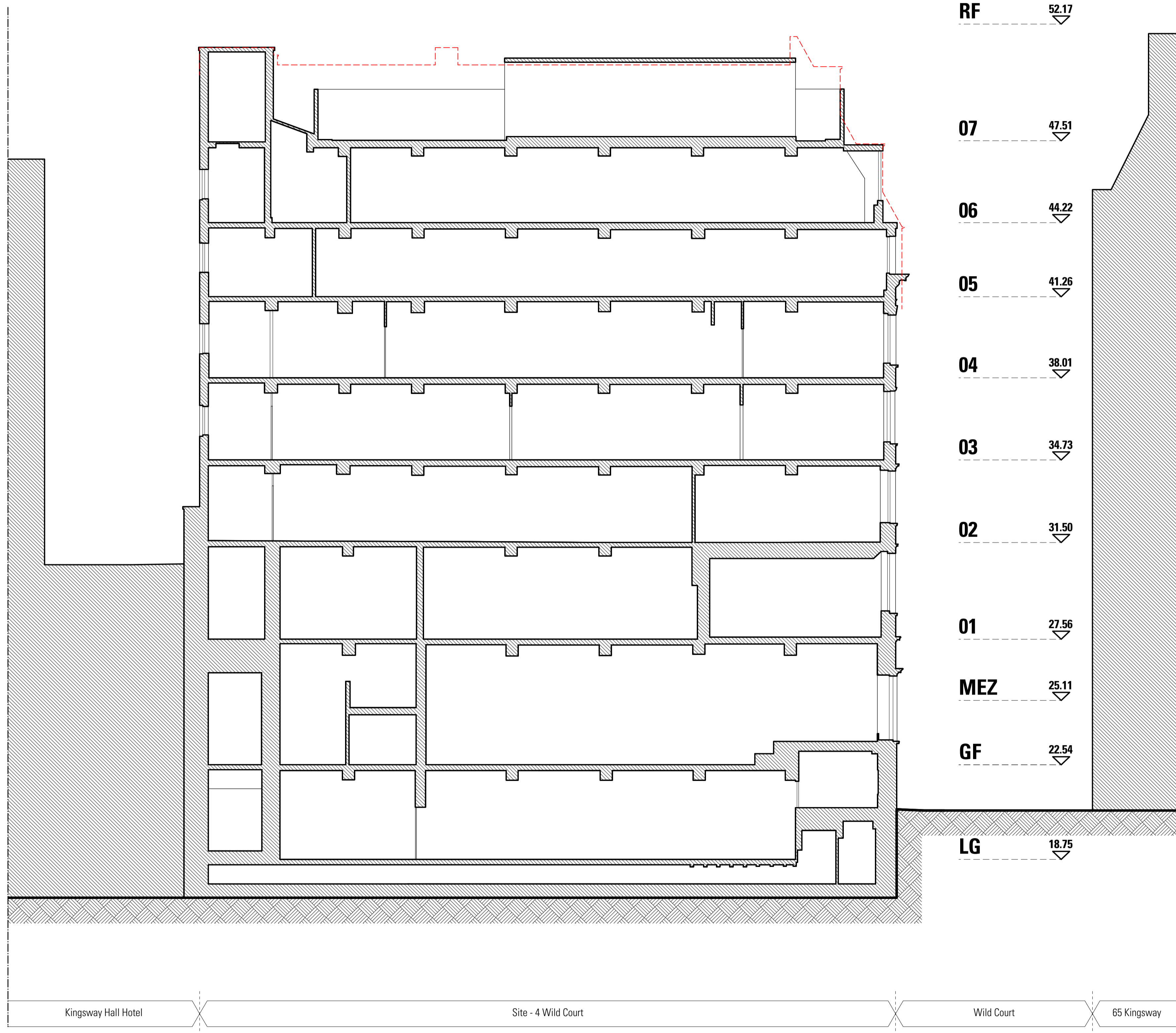
01 Existing Section CC' Scale 1:100 @ A1 / 1:200 @ A3
