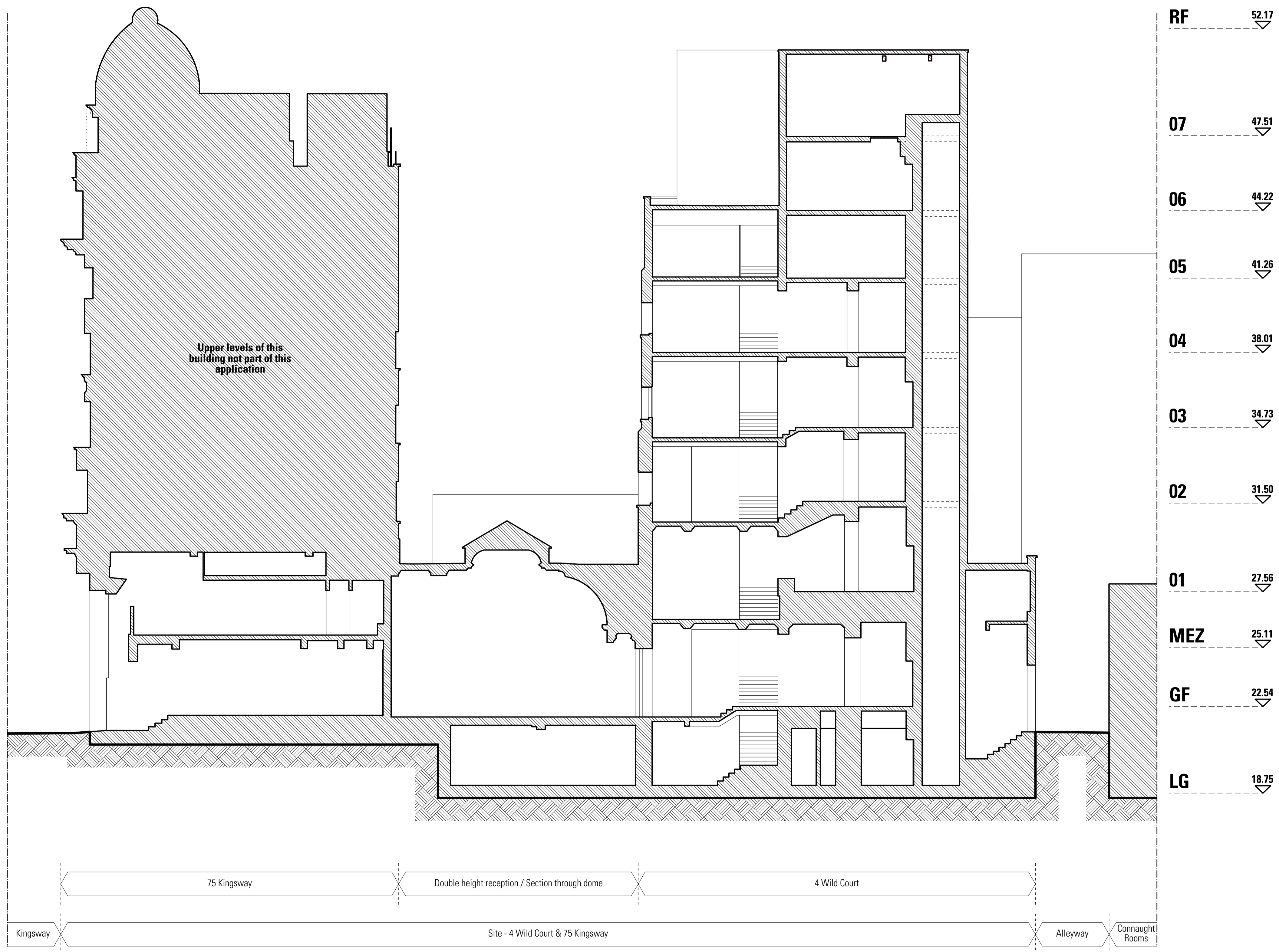
01 Existing Section AA' Scale 1:100 @ A1 / 1:200 @ A3
