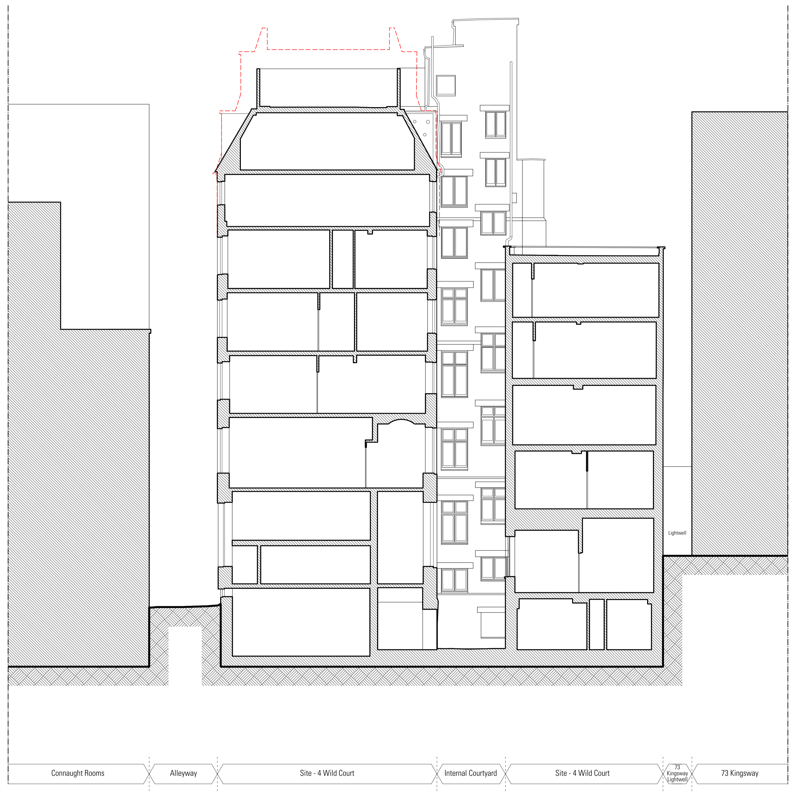
01 Existing Section BB' Scale 1:100 @ A1 / 1:200 @ A3
