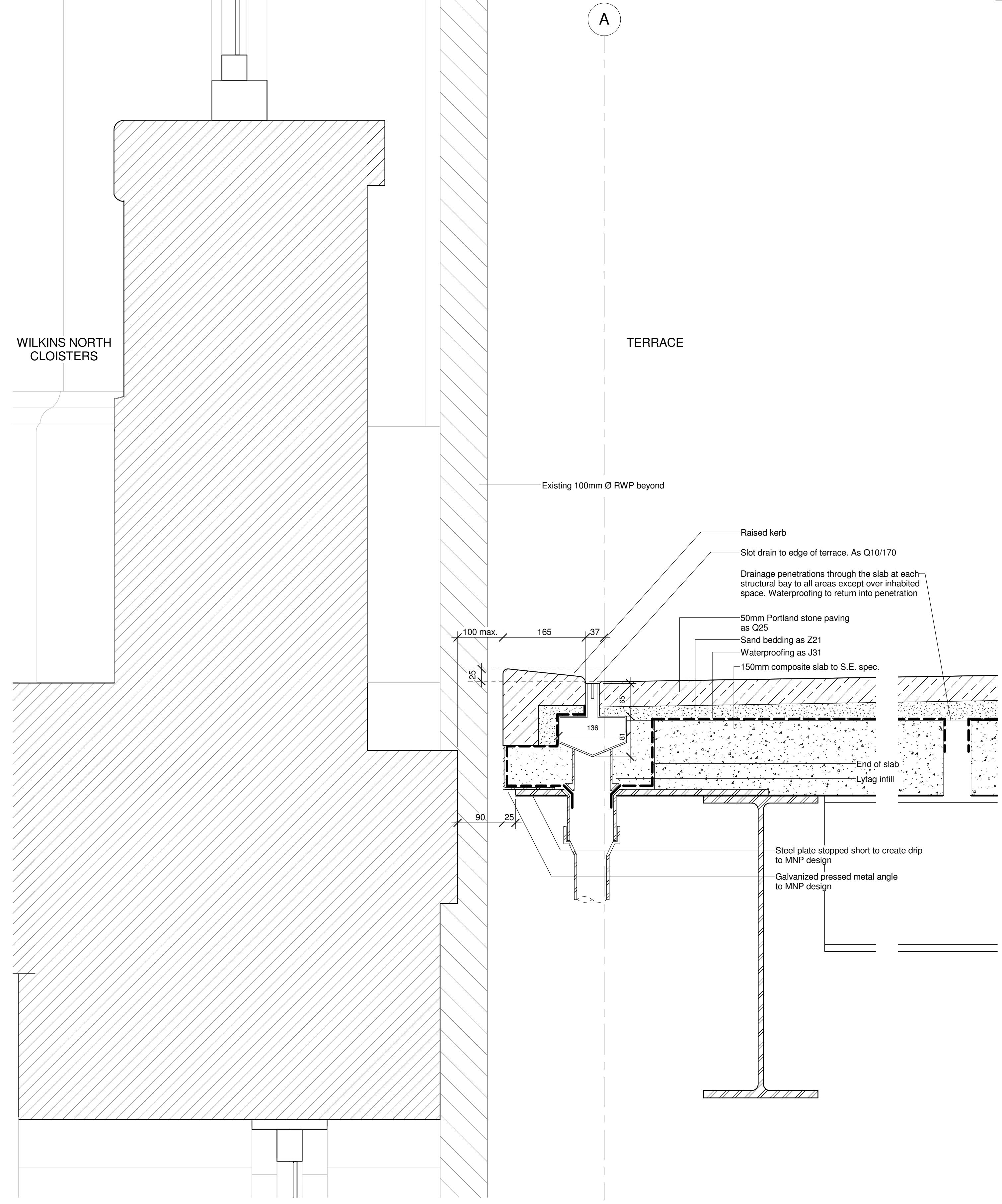
5 636 Terrace Edge Detail - at window 1 : 5
