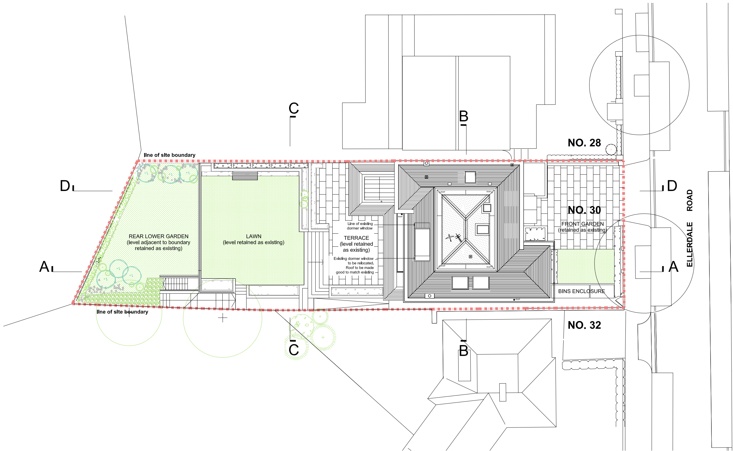
01 Proposed Roof Plan Scale 1 : 100 @ A1 / 1 : 200 @ A3
