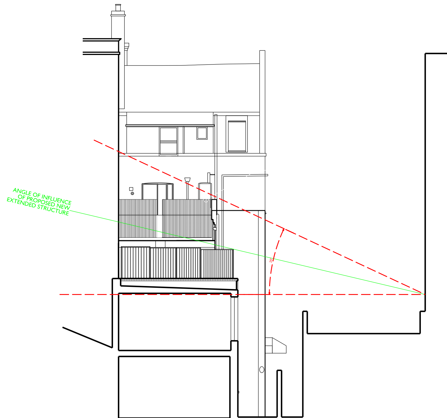
SECTION C-C'
