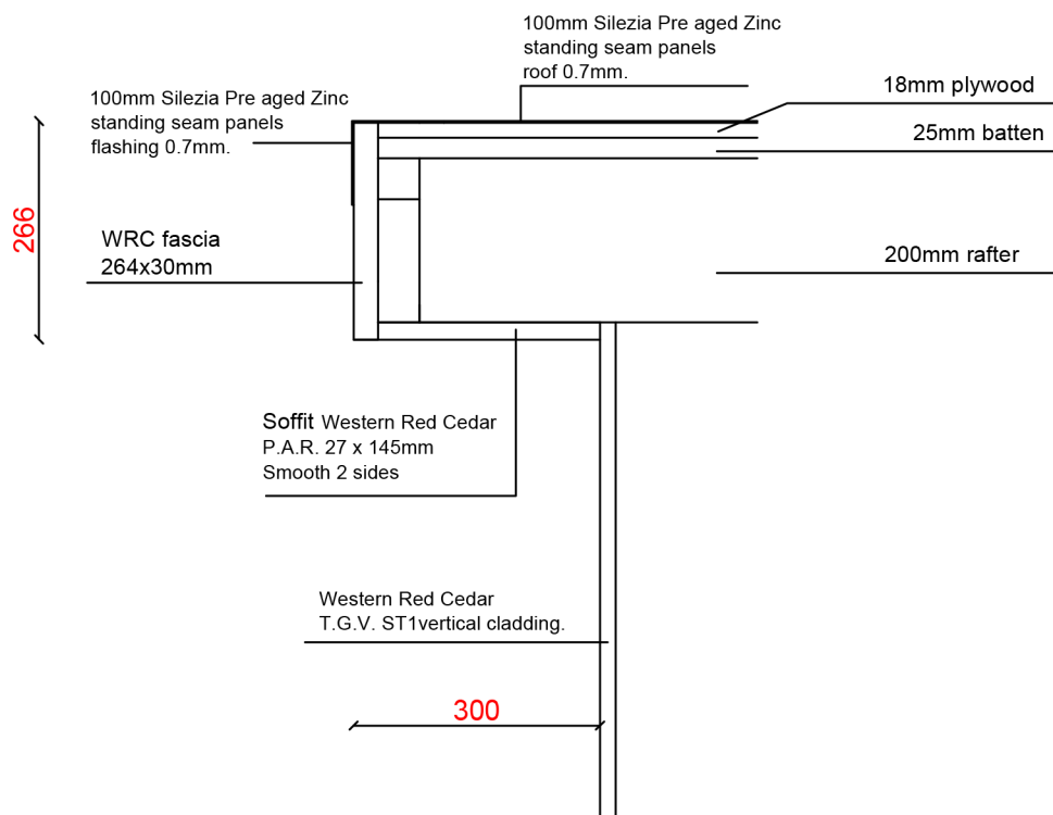
STUDIO ROOF DETAIL 1:10
