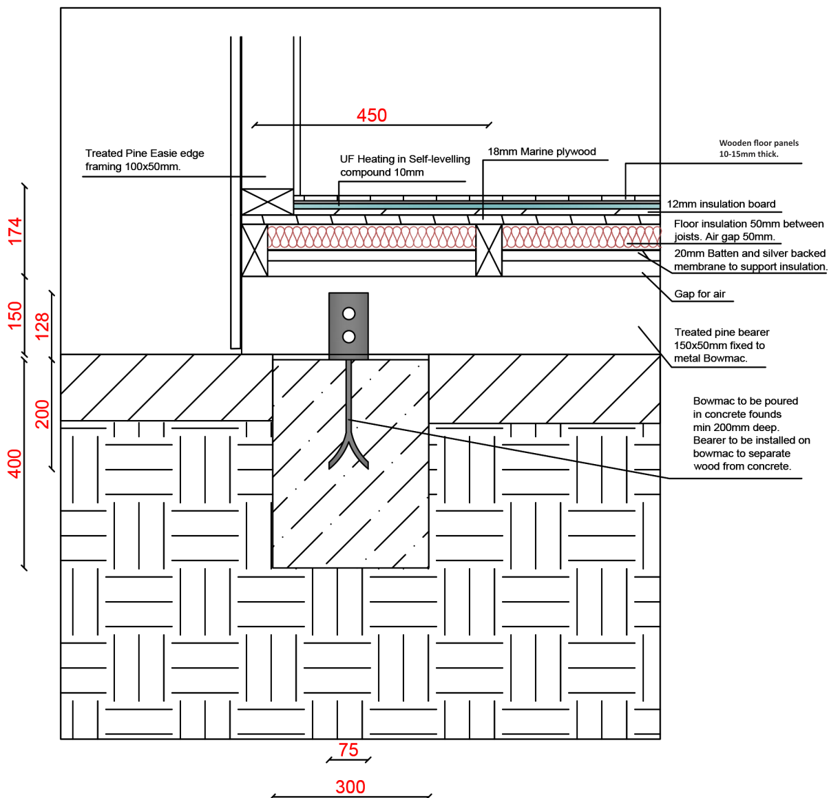
STUDIO FOUNDATION DETAIL 1 SCALE 1:10
