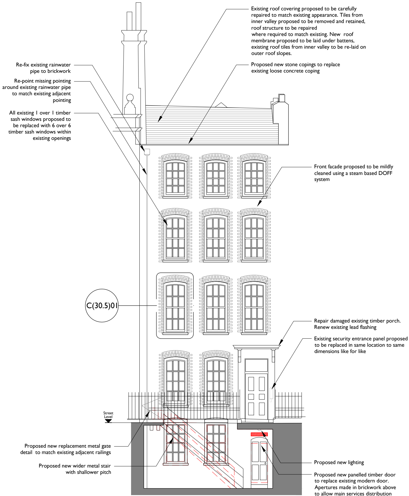
1 220 Proposed Front Elevation 1:100 @ A3
