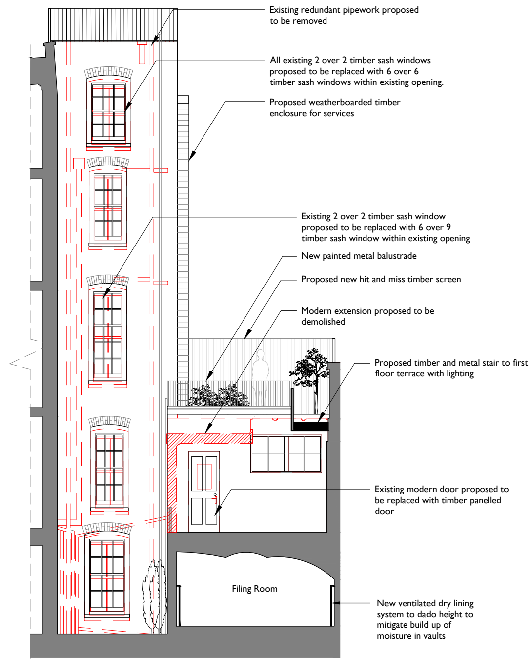
2 220 Proposed Side Elevation 1:100 @ A3
