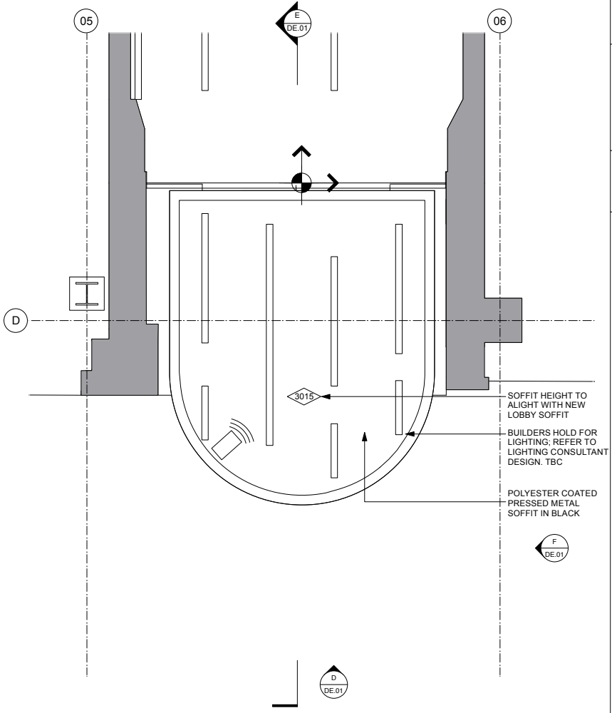
C CANOPY REFLECTED CEILING PLAN DE.01 1:25@A1, 1:50@A3
