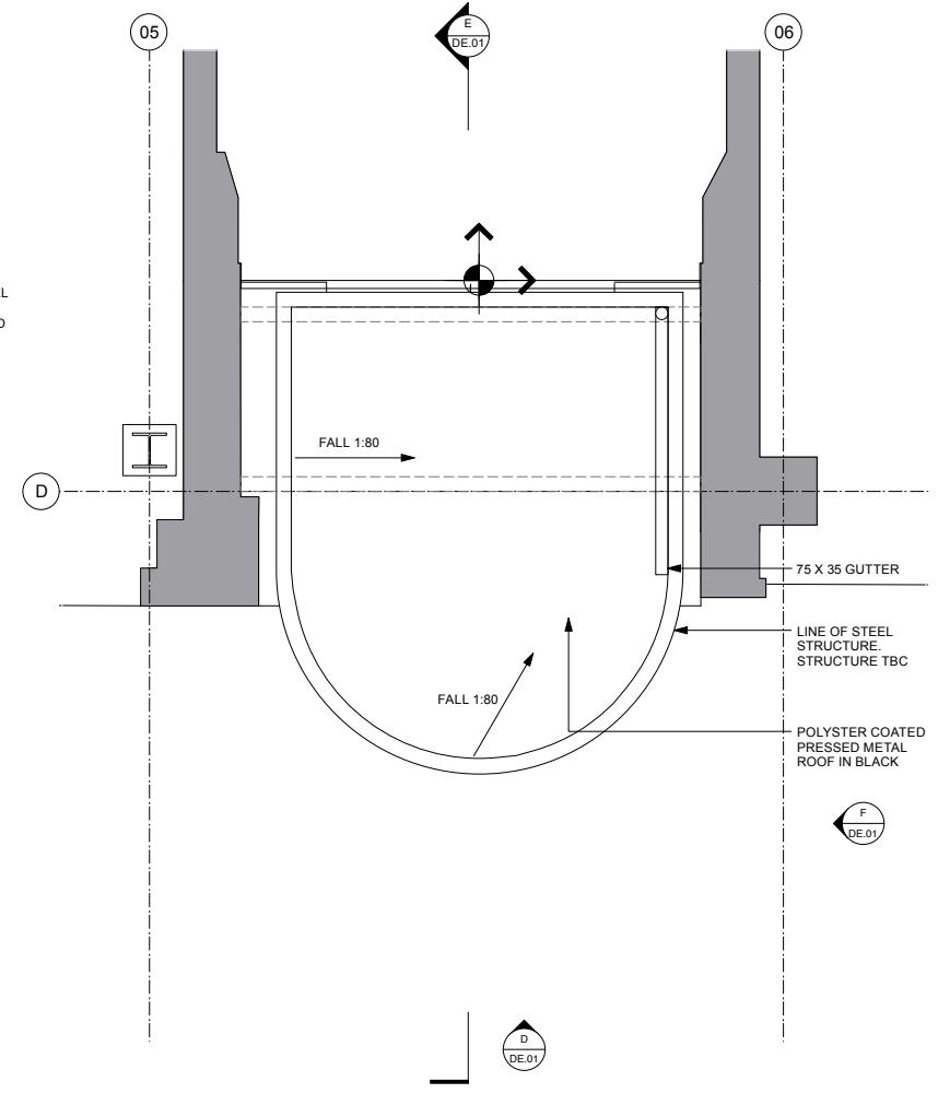
B CANOPY ROOF PLAN DE.01 1:25@A1, 1:50@A3
