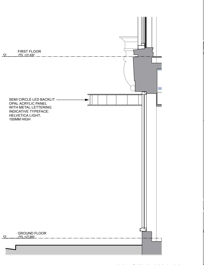
F ENTRY GATES + CANOPY SECTION DE.01 1:25@A1, 1:50@A3
