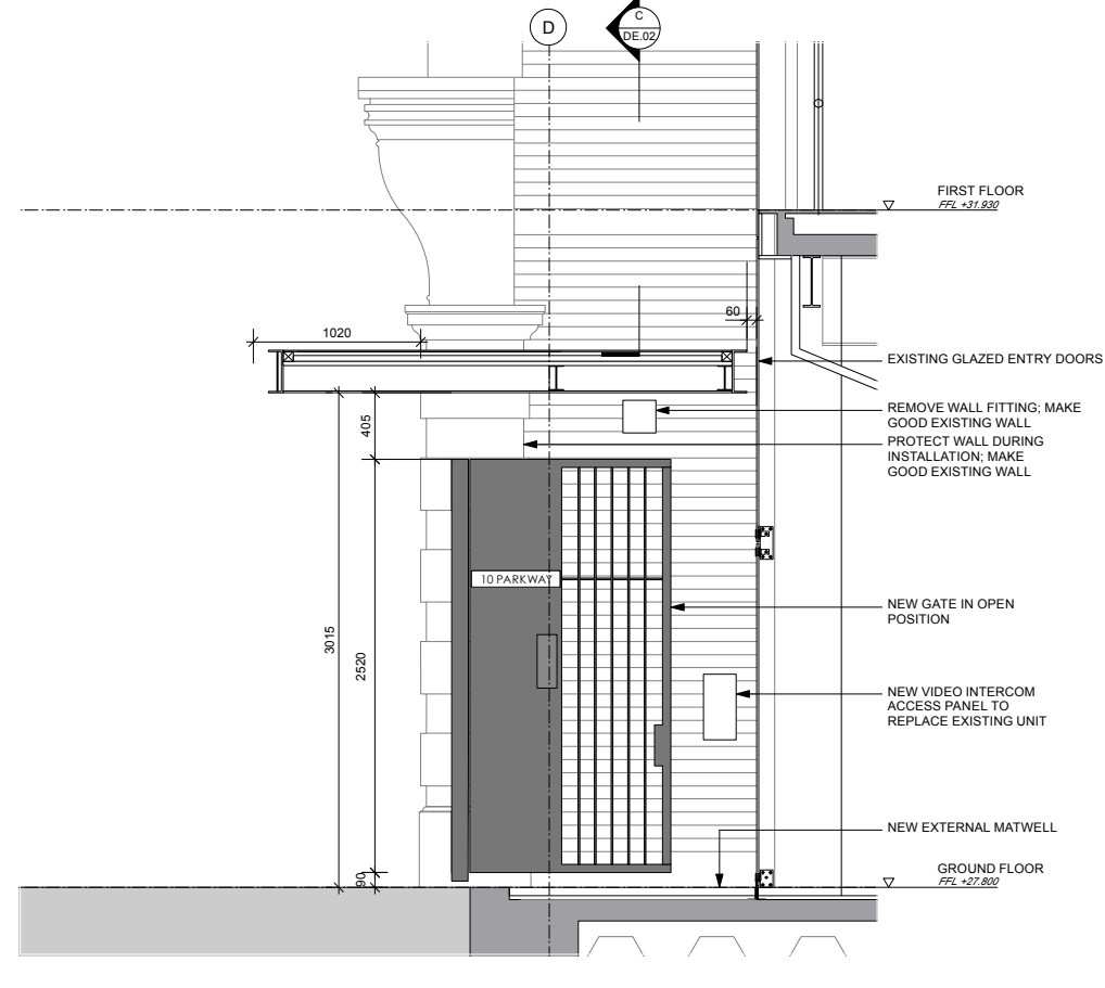
E ENTRY GATES + CANOPY SECTION DE.01 1:25@A1, 1:50@A3
