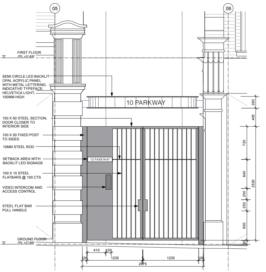
D ENTRY GATES + CANOPY ELEVATION DE.01 1:25@A1, 1:50@A3
