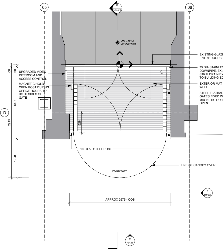
A ENTRY GATES PLAN DE.01 1:25@A1, 1:50@A3
