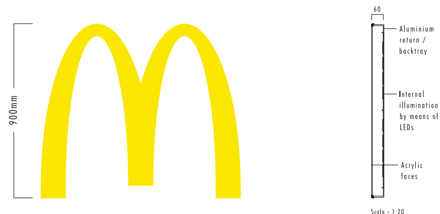
LIM 5 900mm LED ILLUMINATED GOLDEN ARCH scale 1:20
