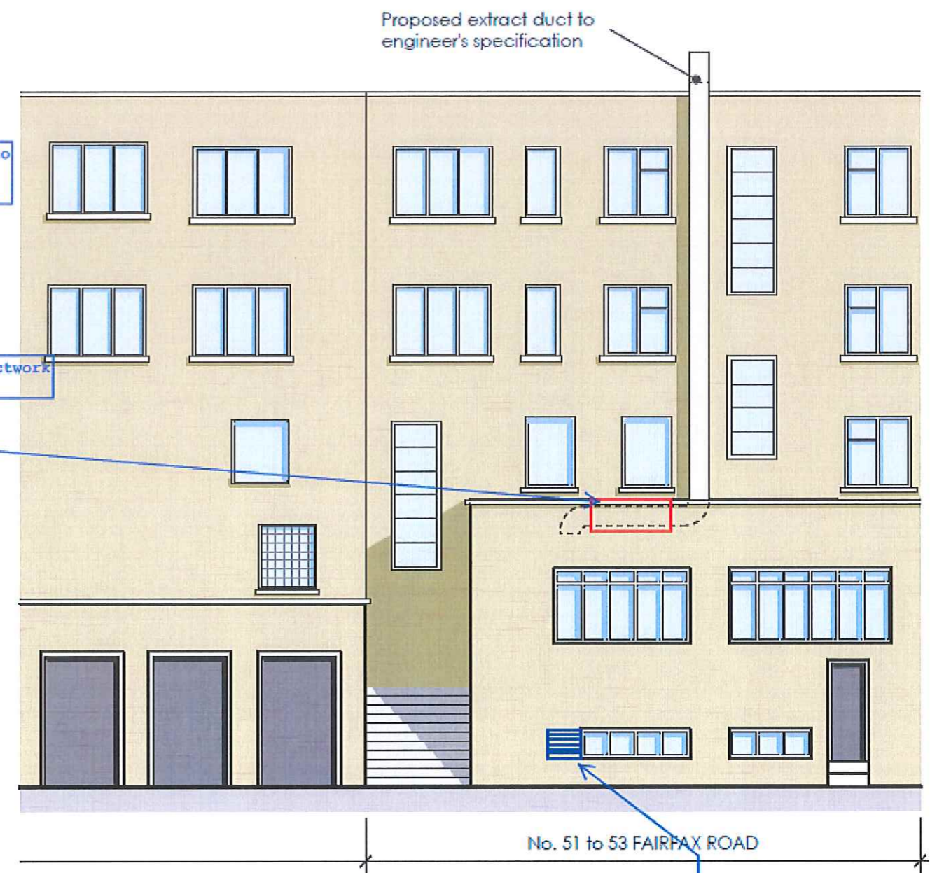
2 121 Proposed Rear Elevation scale 1:100 @ A3
