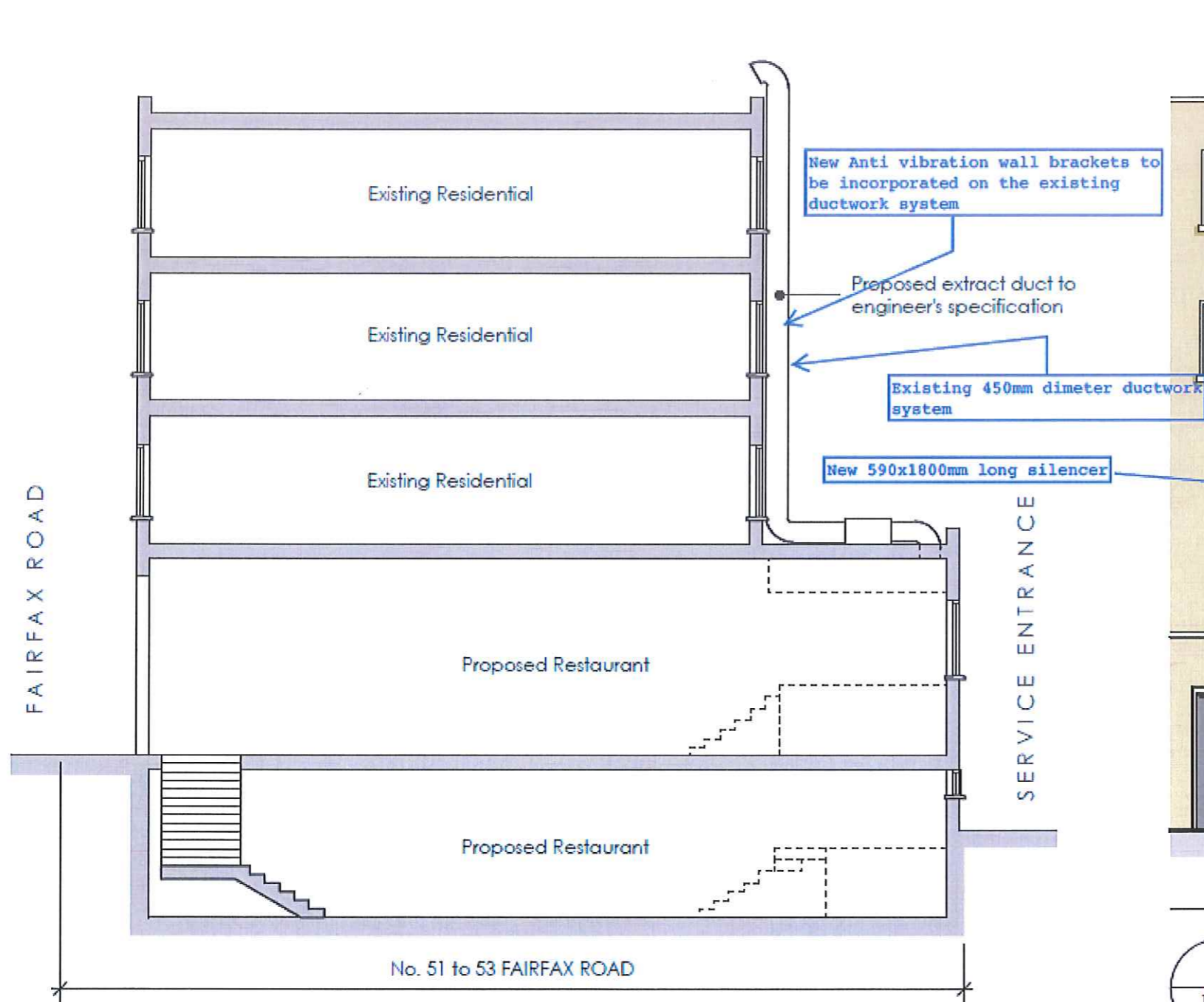
1 121 Proposed Section scale 1:100 @ A3
