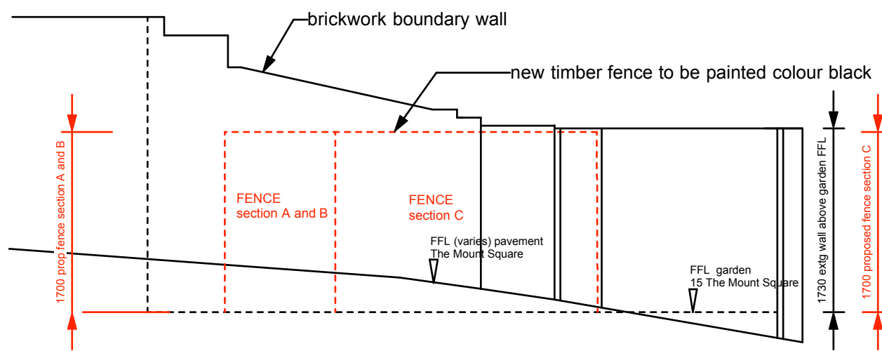
STREET ELEVATION showing line of proposed fence
