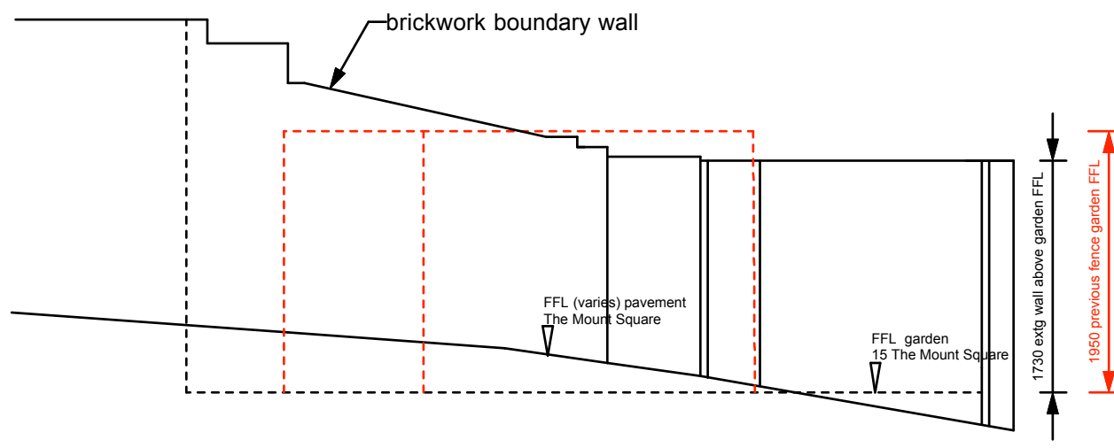
STREET ELEVATION showing line of previously erected fence
