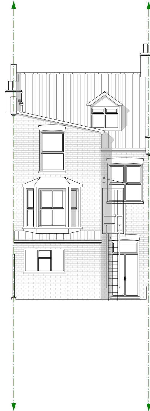
REAR ELEVATION
