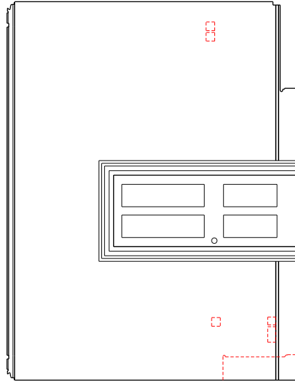
03 Stalwell 18_02_04 Elevation south wall
