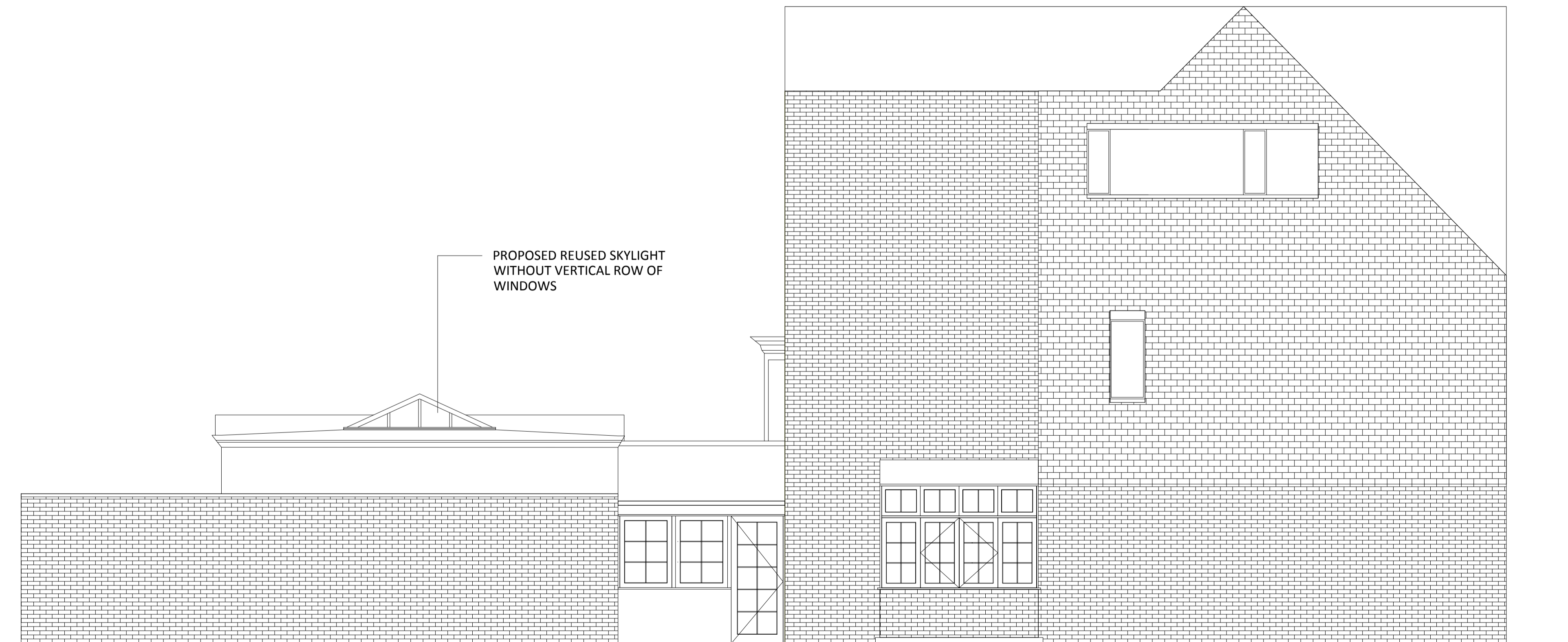
02 PROPOSED SIDE (WEST) ELEVATION 9WG-ID-(14)-01 SCALE 1:50
