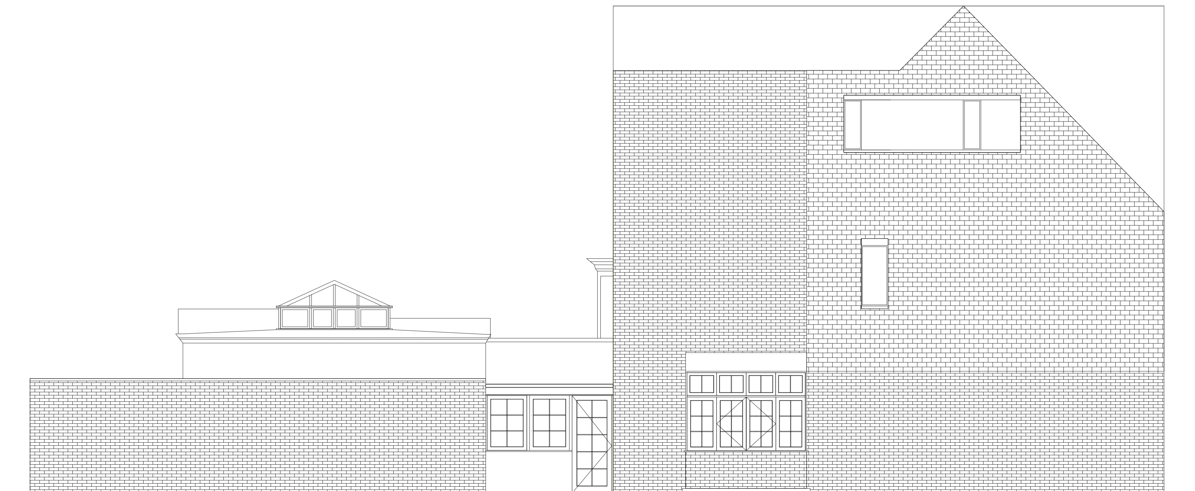
02 EXISTING SIDE (WEST) ELEVATION 9WG-ID-(12)-01 SCALE 1:50
