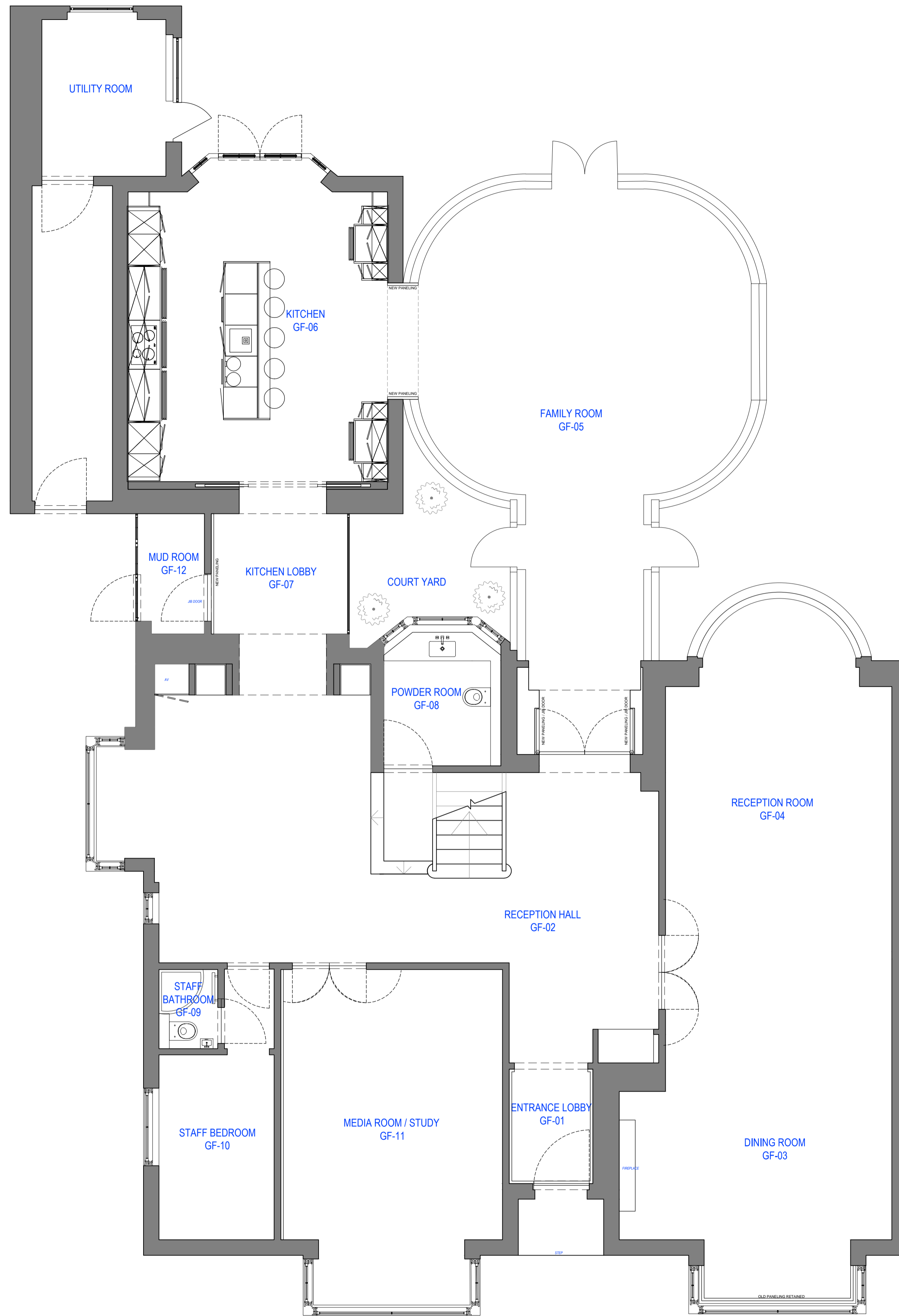
01 PROPOSED GROUND FLOOR PLAN SCALE 1:50
