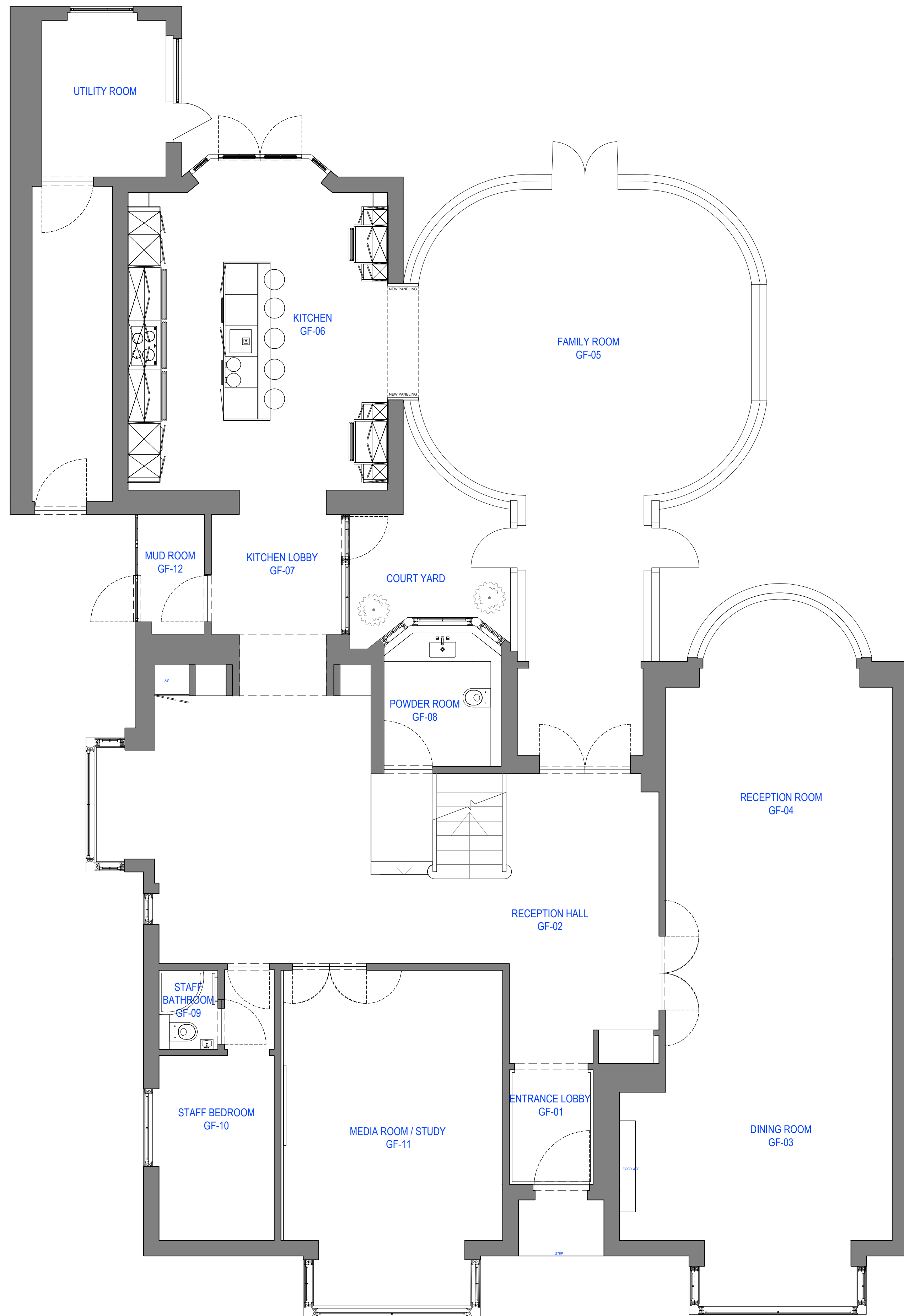
01 EXISTING GROUND FLOOR PLAN SCALE 1:50
