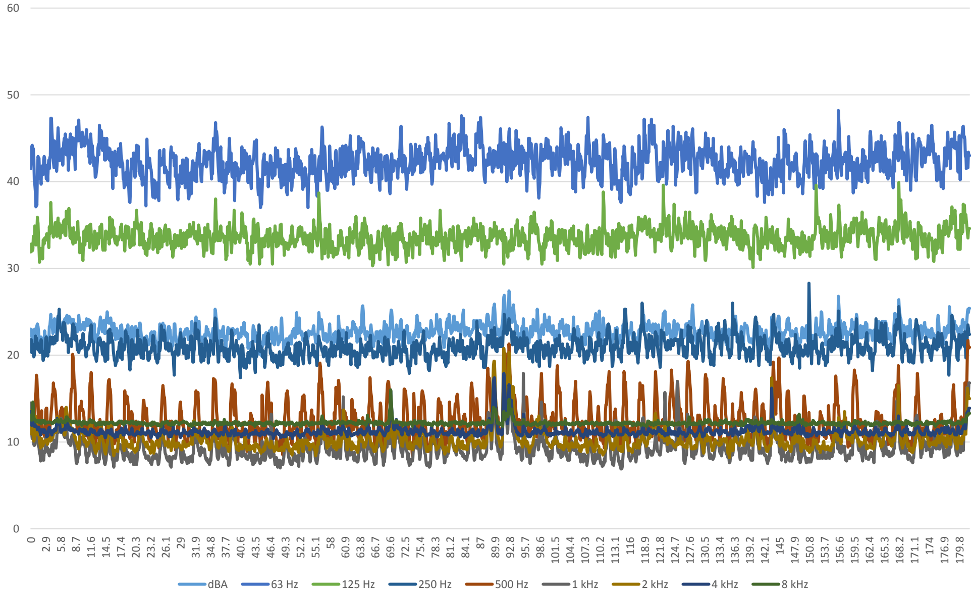
Graph 2: Indoors - Normal operation - approx. 22dBA
