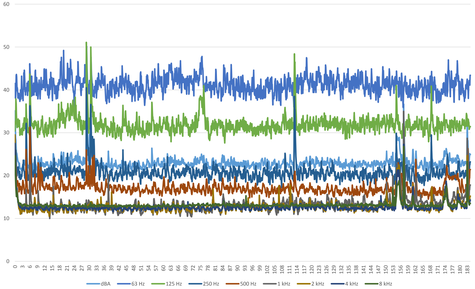
Graph 5: Indoors - Extract Fan off - approx. 22dBA
