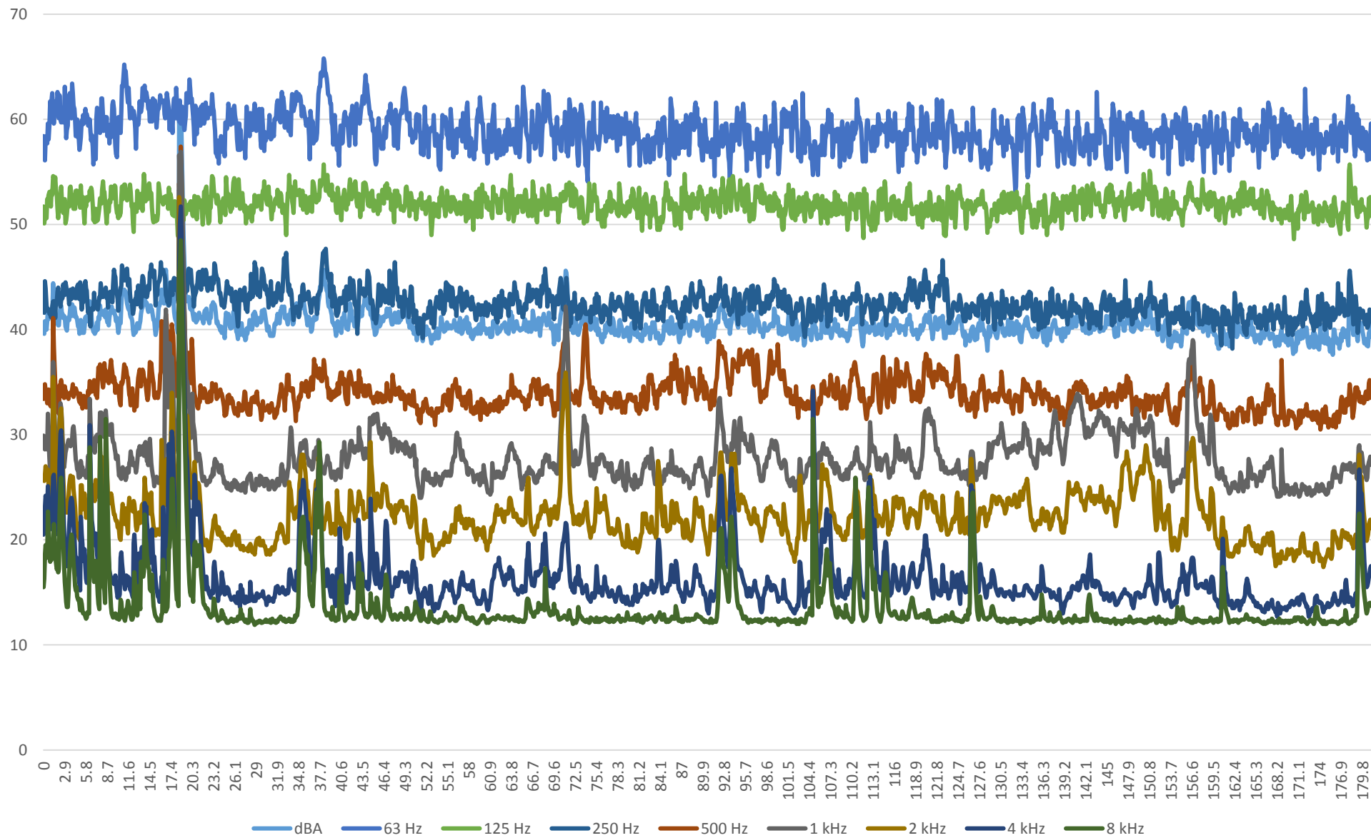
Graph 1: Workshop - Normal operation - approx. 38 - 39dBA
