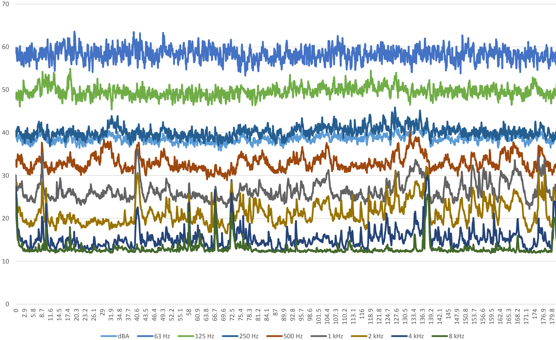
Graph 4: Workshop - Extract Fan off - approx. 37 - 38dBA
