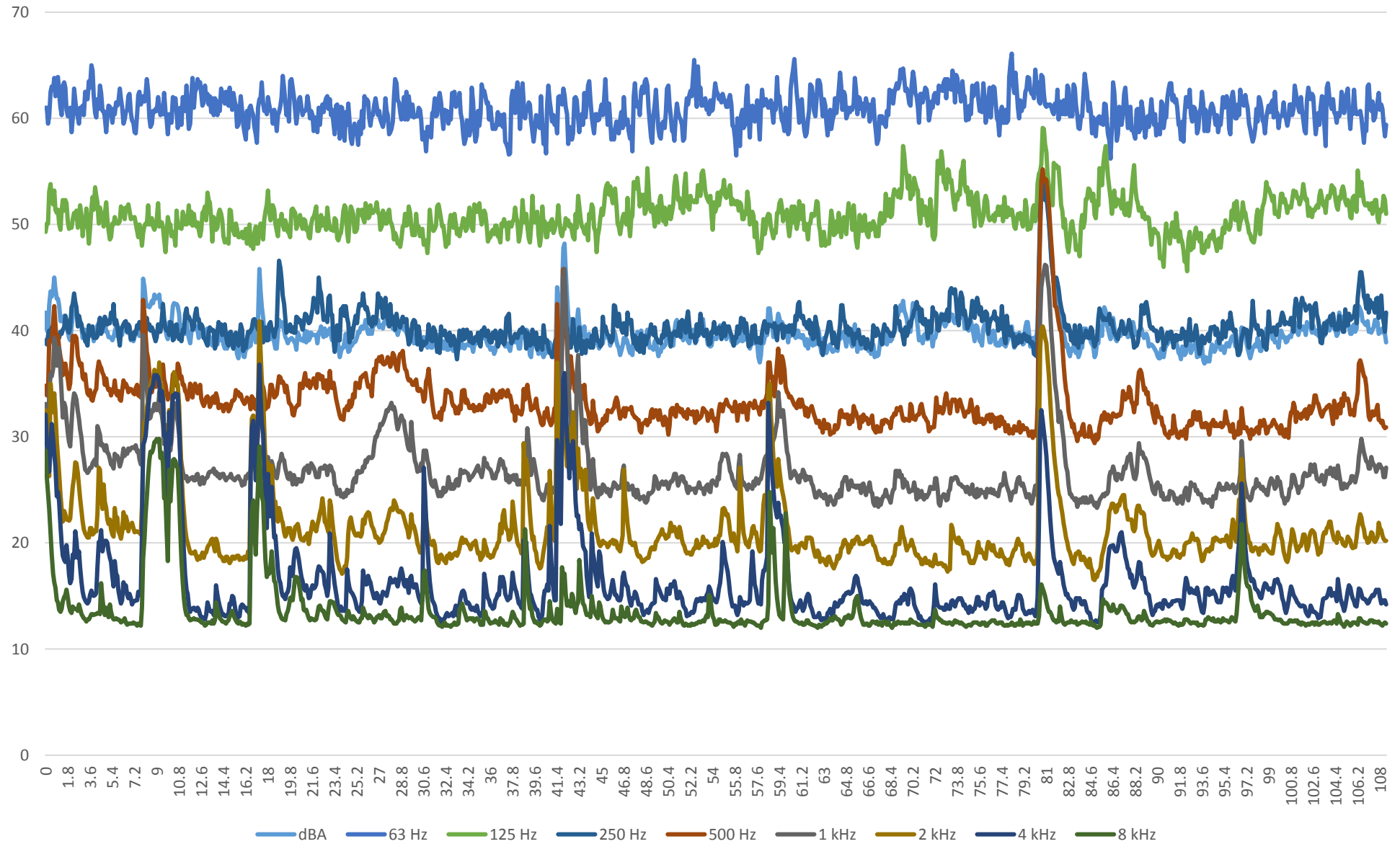
Graph 6: Workshop - Extract Fan off then on
