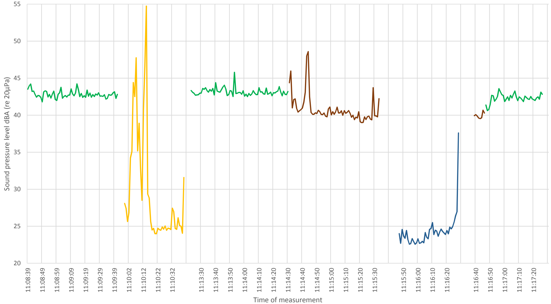
Graph 2 - Sound Level in Flat B with plant operating and inoperative Measured 18 th July 2016
