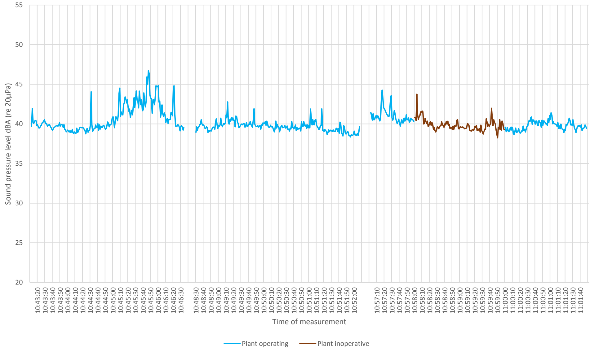
Graph 1 - Sound Level in Flat C with plant operating and inoperative Measured 18 th July 2016
